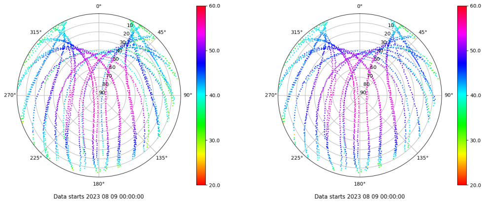
Skyplot for station LPAL. Signal to Noise S1C Data file LPAL00ESP_R_2023221.xtr Skyplot for station LPAL. Signal to Noise S2C Data file LPAL00ESP_R_2023221.xtr
