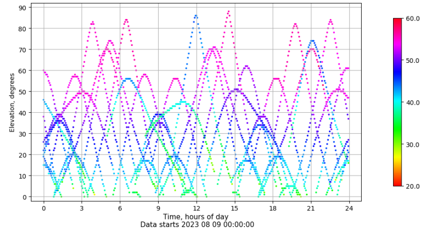
Time-elevation plot for station LPAL. Signal to Noise S1C Data file LPAL00ESP_R_2023221.xtr
