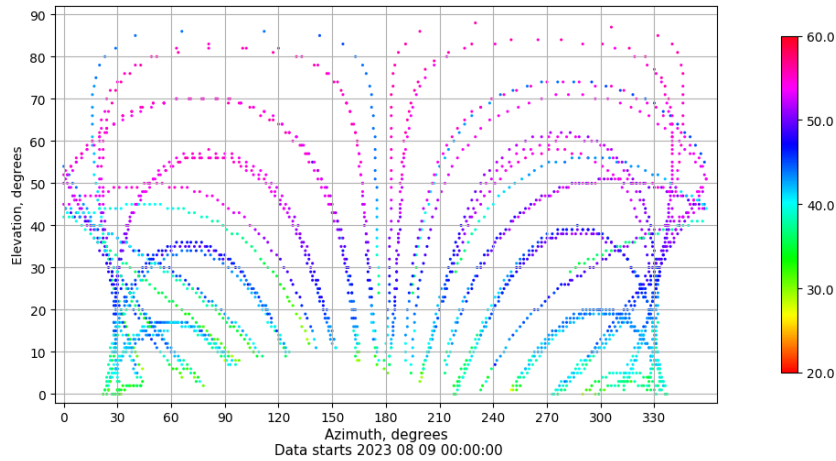
Azimuth-elevation plot for station LPAL. Signal to Noise S1C Data file LPAL00ESP_R_2023221.xtr
