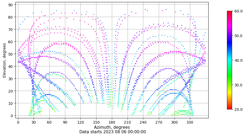
Azimuth-elevation plot for station LPAL. Signal to Noise S1C Data file LPAL00ESP_R_2023218.xtr
