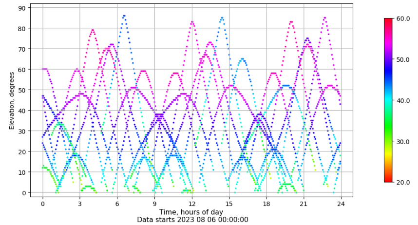
Time-elevation plot for station LPAL. Signal to Noise S1C Data file LPAL00ESP_R_2023218.xtr
