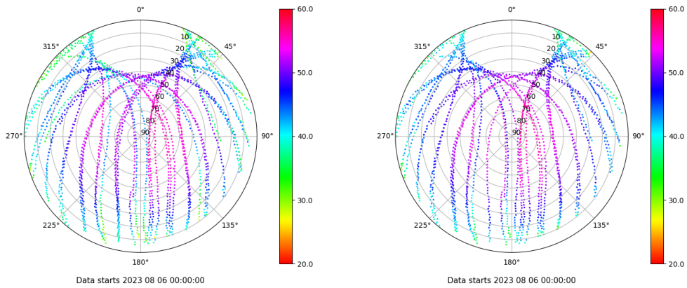
Skyplot for station LPAL. Signal to Noise S1C Data file LPAL00ESP_R_2023218.xtr Skyplot for station LPAL. Signal to Noise S2C Data file LPAL00ESP_R_2023218.xtr
