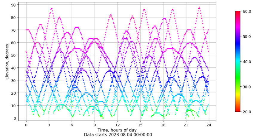
Time-elevation plot for station LPAL. Signal to Noise S1C Data file LPAL00ESP_R_2023216.xtr
