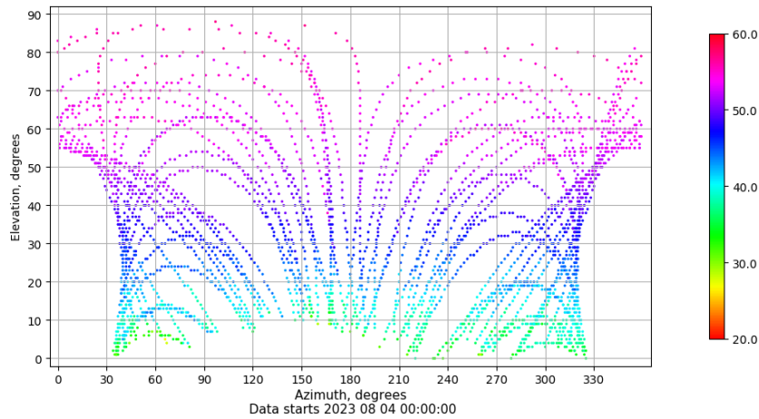
Azimuth-elevation plot for station LPAL. Signal to Noise S1C Data file LPAL00ESP_R_2023216.xtr
