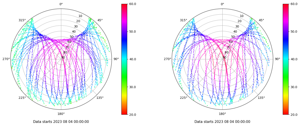
Skyplot for station LPAL. Signal to Noise S1C Data file LPAL00ESP_R_2023216.xtr Skyplot for station LPAL. Signal to Noise S2S Data file LPAL00ESP_R_2023216.xtr
