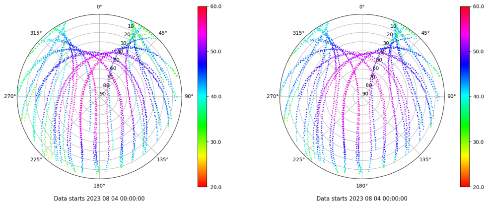
Skyplot for station LPAL. Signal to Noise S1C Data file LPAL00ESP_R_2023216.xtr Skyplot for station LPAL. Signal to Noise S2C Data file LPAL00ESP_R_2023216.xtr
