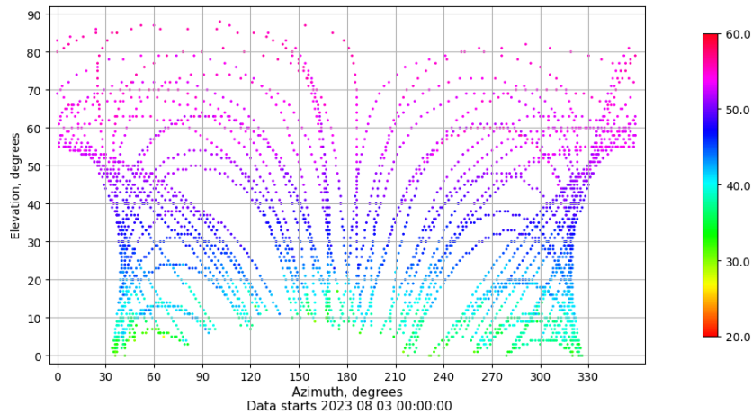
Azimuth-elevation plot for station LPAL. Signal to Noise S1C Data file LPAL00ESP_R_2023215.xtr
