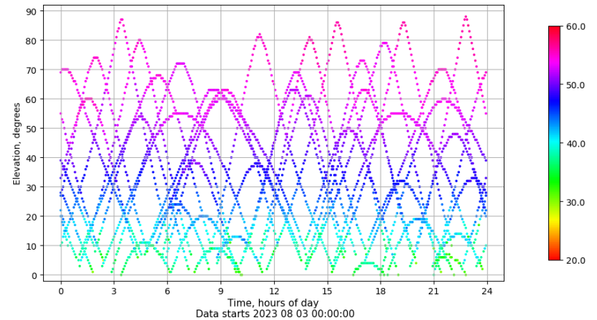
Time-elevation plot for station LPAL. Signal to Noise S1C Data file LPAL00ESP_R_2023215.xtr
