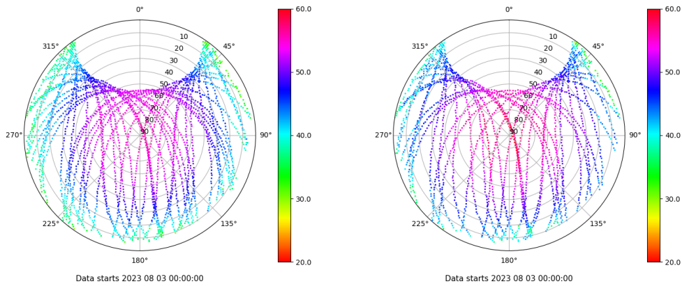
Skyplot for station LPAL. Signal to Noise S1C Data file LPAL00ESP_R_2023215.xtr Skyplot for station LPAL. Signal to Noise S2S Data file LPAL00ESP_R_2023215.xtr
