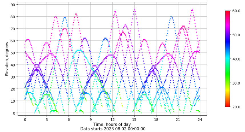
Time-elevation plot for station LPAL. Signal to Noise S1C Data file LPAL00ESP_R_2023214.xtr
