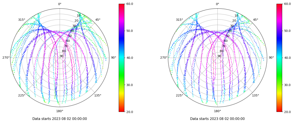
Skyplot for station LPAL. Signal to Noise S1C Data file LPAL00ESP_R_2023214.xtr Skyplot for station LPAL. Signal to Noise S2C Data file LPAL00ESP_R_2023214.xtr
