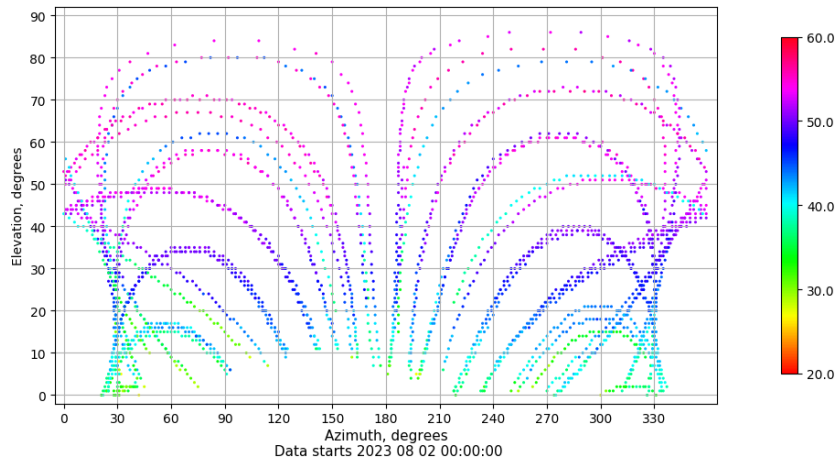
Azimuth-elevation plot for station LPAL. Signal to Noise S1C Data file LPAL00ESP_R_2023214.xtr
