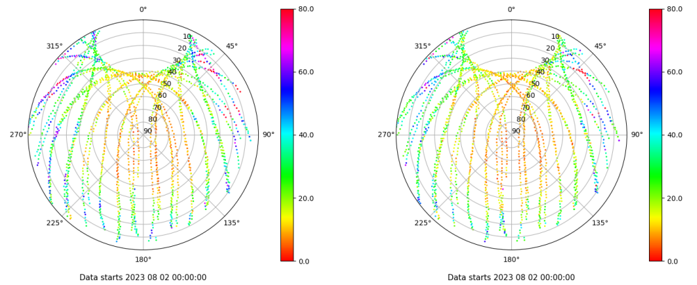
Skyplot for station LPAL. Parameter M1C Data file LPAL00ESP_R_2023214.xtr Skyplot for station LPAL. Parameter M2C Data file LPAL00ESP_R_2023214.xtr
