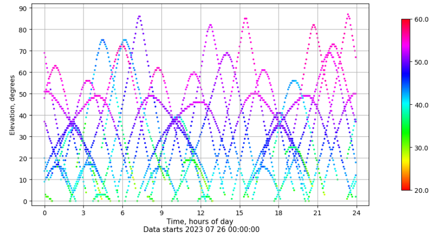
Time-elevation plot for station LPAL. Signal to Noise S1C Data file LPAL00ESP_R_2023207.xtr
