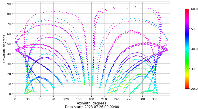
Azimuth-elevation plot for station LPAL. Signal to Noise S1C Data file LPAL00ESP_R_2023207.xtr
