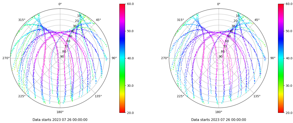
Skyplot for station LPAL. Signal to Noise S1C Data file LPAL00ESP_R_2023207.xtr Skyplot for station LPAL. Signal to Noise S2C Data file LPAL00ESP_R_2023207.xtr
