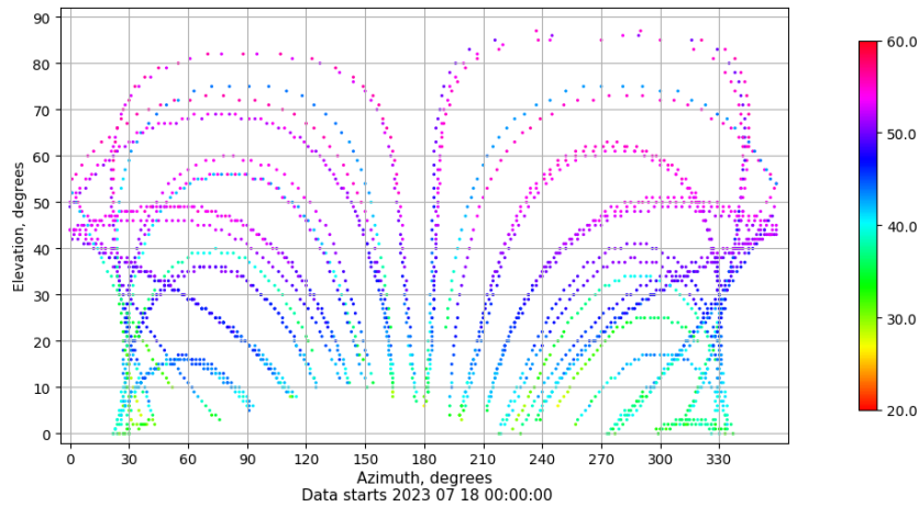
Azimuth-elevation plot for station LPAL. Signal to Noise S1C Data file LPAL00ESP_R_2023199.xtr
