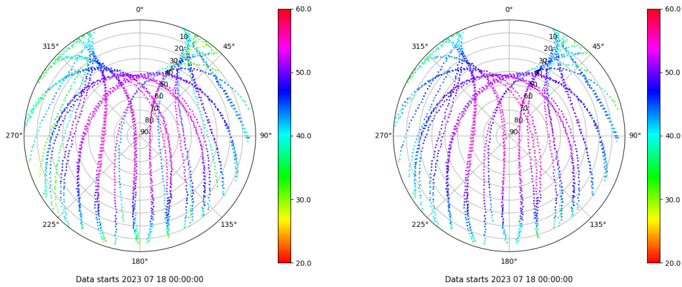
Skyplot for station LPAL. Signal to Noise S1C Data file LPAL00ESP_R_2023199.xtr Skyplot for station LPAL. Signal to Noise S2C Data file LPAL00ESP_R_2023199.xtr
