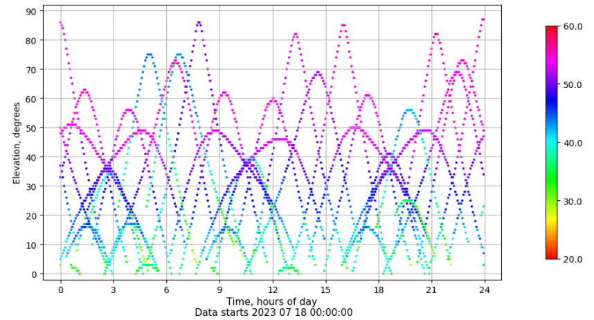
Time-elevation plot for station LPAL. Signal to Noise S1C Data file LPAL00ESP_R_2023199.xtr
