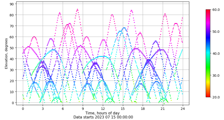
Time-elevation plot for station LPAL. Signal to Noise S1C Data file LPAL00ESP_R_2023196.xtr
