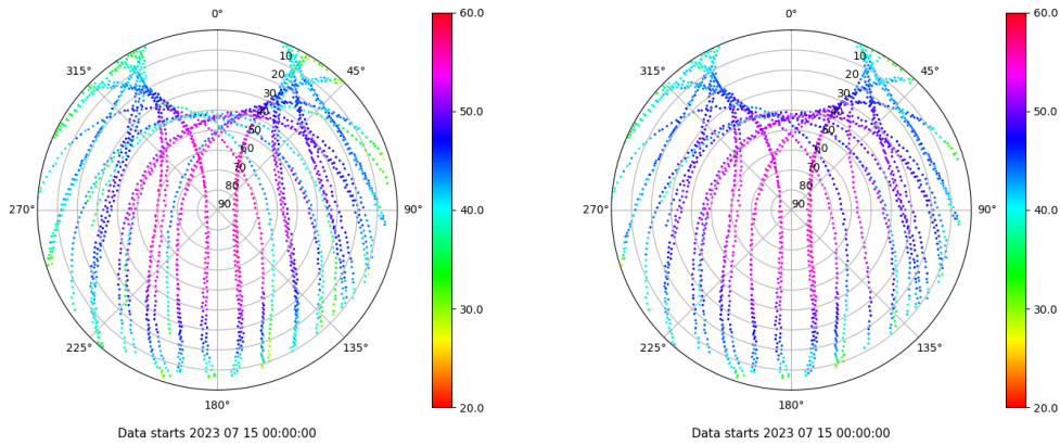
Skyplot for station LPAL. Signal to Noise S1C Data file LPAL00ESP_R_2023196.xtr Skyplot for station LPAL. Signal to Noise S2C Data file LPAL00ESP_R_2023196.xtr
