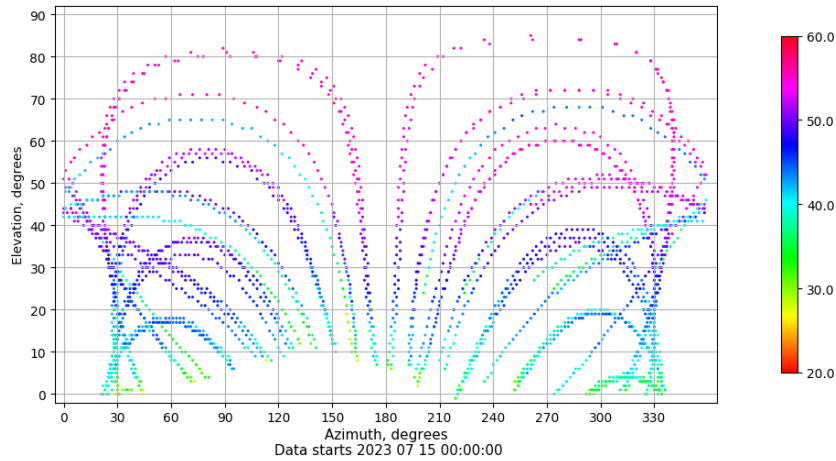
Azimuth-elevation plot for station LPAL. Signal to Noise S1C Data file LPAL00ESP_R_2023196.xtr
