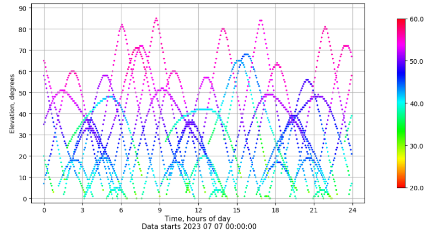
Time-elevation plot for station LPAL. Signal to Noise S1C Data file LPAL00ESP_R_2023188.xtr
