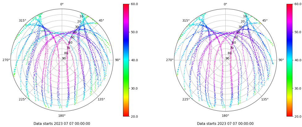
Skyplot for station LPAL. Signal to Noise S1C Data file LPAL00ESP_R_2023188.xtr Skyplot for station LPAL. Signal to Noise S2C Data file LPAL00ESP_R_2023188.xtr
