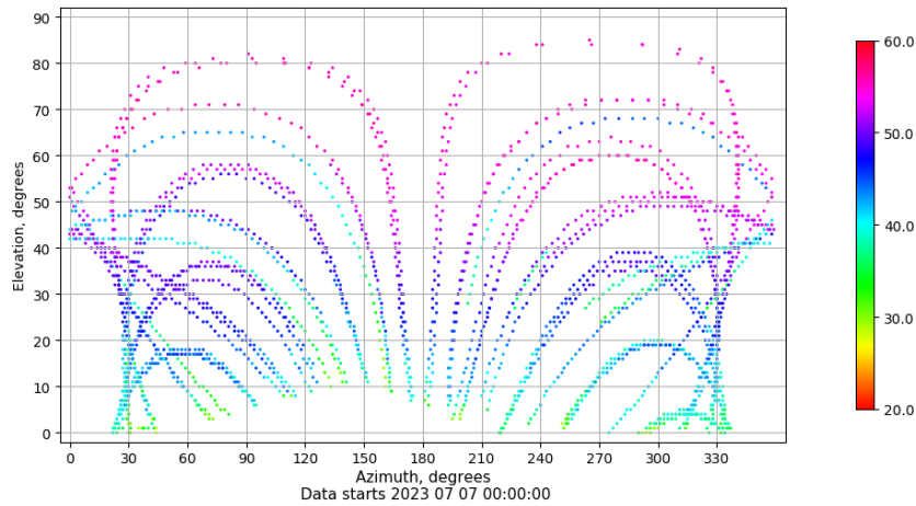
Azimuth-elevation plot for station LPAL. Signal to Noise S1C Data file LPAL00ESP_R_2023188.xtr
