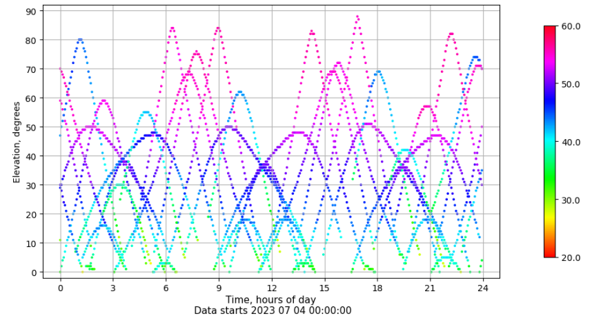
Time-elevation plot for station LPAL. Signal to Noise S1C Data file LPAL00ESP_R_2023185.xtr
