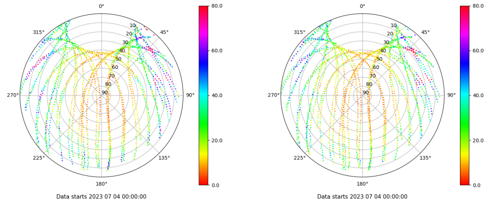
Skyplot for station LPAL. Parameter M1C Data file LPAL00ESP_R_2023185.xtr Skyplot for station LPAL. Parameter M2C Data file LPAL00ESP_R_2023185.xtr
