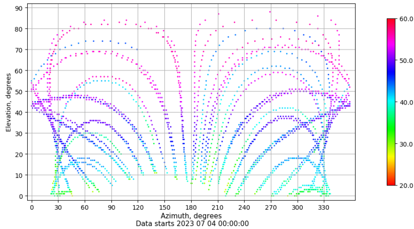
Azimuth-elevation plot for station LPAL. Signal to Noise S1C Data file LPAL00ESP_R_2023185.xtr
