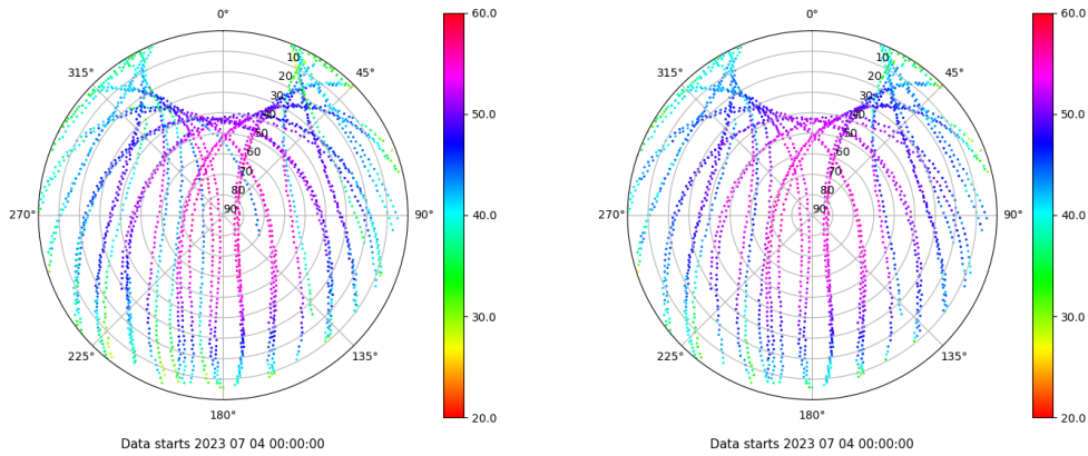
Skyplot for station LPAL. Signal to Noise S1C Data file LPAL00ESP_R_2023185.xtr Skyplot for station LPAL. Signal to Noise S2C Data file LPAL00ESP_R_2023185.xtr
