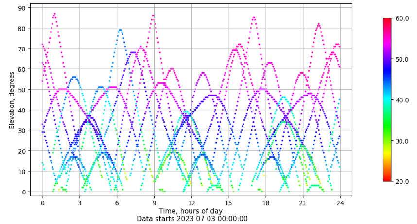
Time-elevation plot for station LPAL. Signal to Noise S1C Data file LPAL00ESP_R_2023184.xtr
