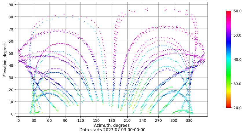
Azimuth-elevation plot for station LPAL. Signal to Noise S1C Data file LPAL00ESP_R_2023184.xtr
