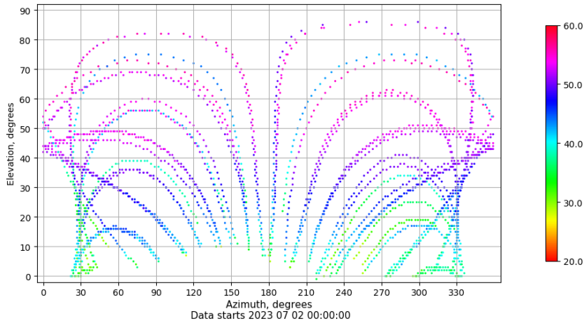
Azimuth-elevation plot for station LPAL. Signal to Noise S1C Data file LPAL00ESP_R_2023183.xtr
