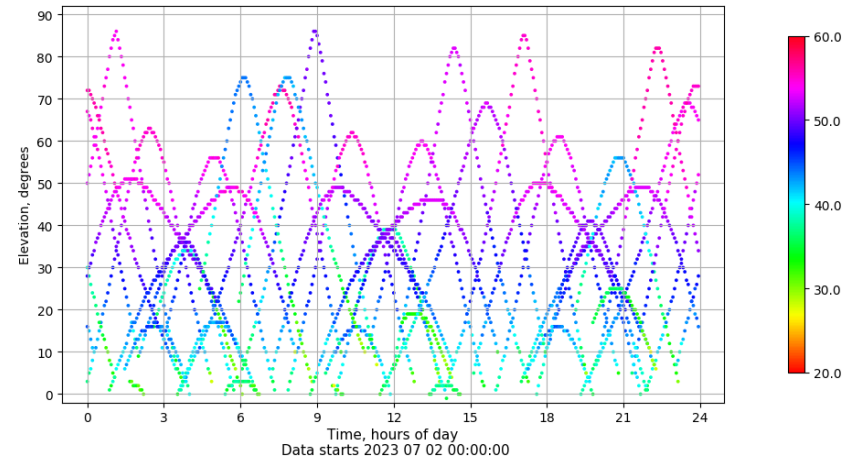
Time-elevation plot for station LPAL. Signal to Noise S1C Data file LPAL00ESP_R_2023183.xtr
