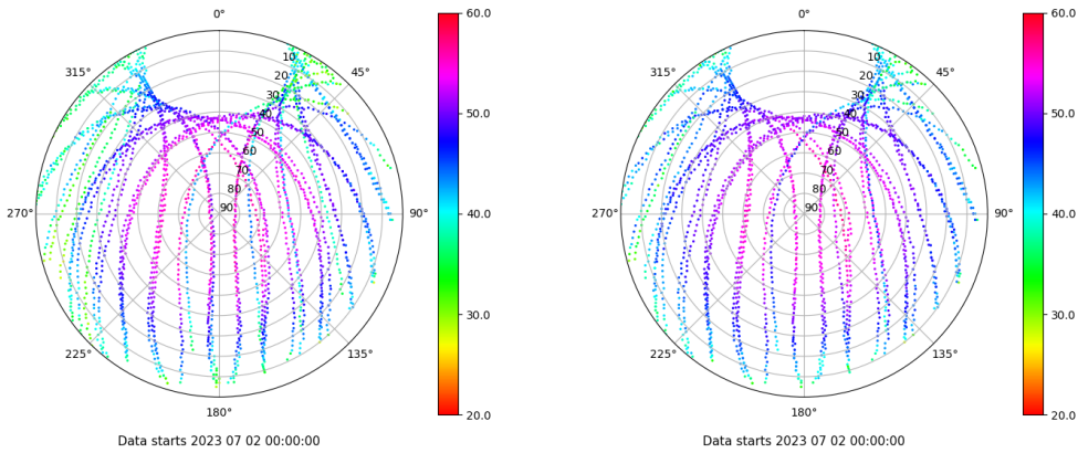
Skyplot for station LPAL. Signal to Noise S1C Data file LPAL00ESP_R_2023183.xtr Skyplot for station LPAL. Signal to Noise S2C Data file LPAL00ESP_R_2023183.xtr
