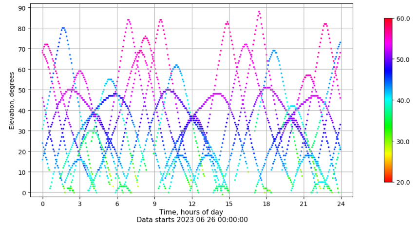
Time-elevation plot for station LPAL. Signal to Noise S1C Data file LPAL00ESP_R_2023177.xtr
