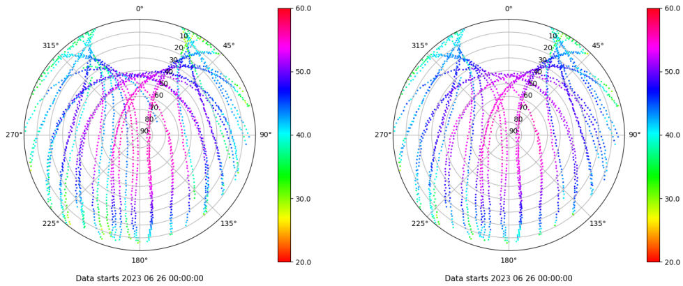
Skyplot for station LPAL. Signal to Noise S1C Data file LPAL00ESP_R_2023177.xtr Skyplot for station LPAL. Signal to Noise S2C Data file LPAL00ESP_R_2023177.xtr
