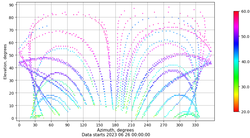
Azimuth-elevation plot for station LPAL. Signal to Noise S1C Data file LPAL00ESP_R_2023177.xtr
