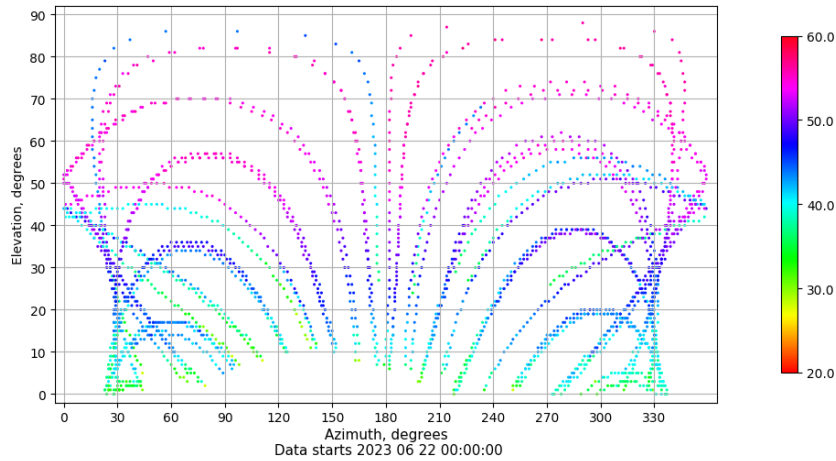
Azimuth-elevation plot for station LPAL. Signal to Noise S1C Data file LPAL00ESP_R_2023173.xtr
