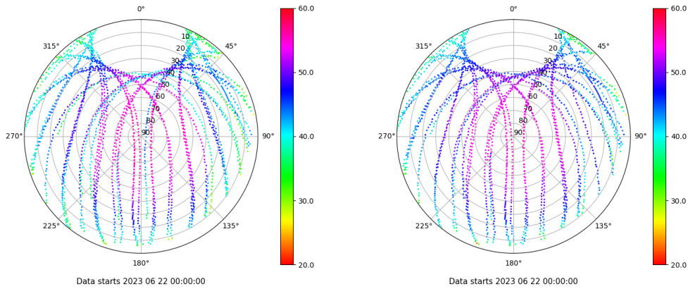
Skyplot for station LPAL. Signal to Noise S1C Data file LPAL00ESP_R_2023173.xtr Skyplot for station LPAL. Signal to Noise S2C Data file LPAL00ESP_R_2023173.xtr
