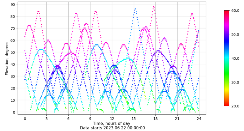
Time-elevation plot for station LPAL. Signal to Noise S1C Data file LPAL00ESP_R_2023173.xtr
