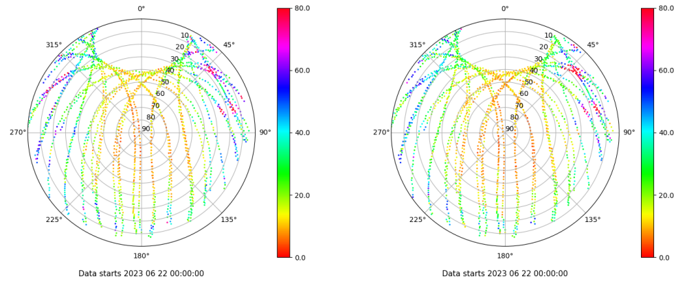
Skyplot for station LPAL. Parameter M1C Data file LPAL00ESP_R_2023173.xtr Skyplot for station LPAL. Parameter M2C Data file LPAL00ESP_R_2023173.xtr
