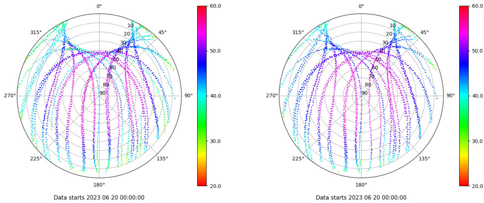
Skyplot for station LPAL. Signal to Noise S1C Data file LPAL00ESP_R_2023171.xtr Skyplot for station LPAL. Signal to Noise S2C Data file LPAL00ESP_R_2023171.xtr
