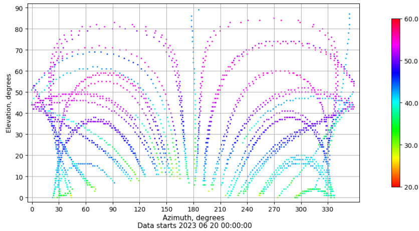
Azimuth-elevation plot for station LPAL. Signal to Noise S1C Data file LPAL00ESP_R_2023171.xtr
