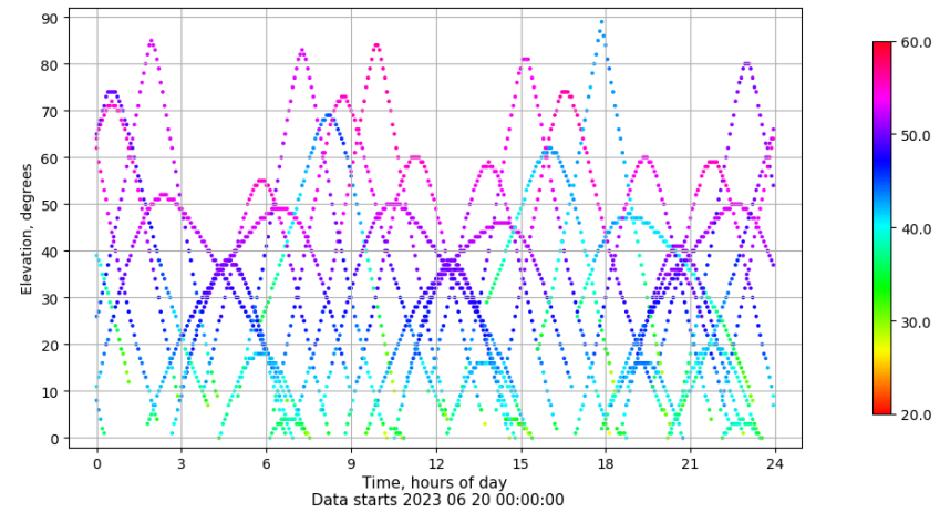
Time-elevation plot for station LPAL. Signal to Noise S1C Data file LPAL00ESP_R_2023171.xtr
