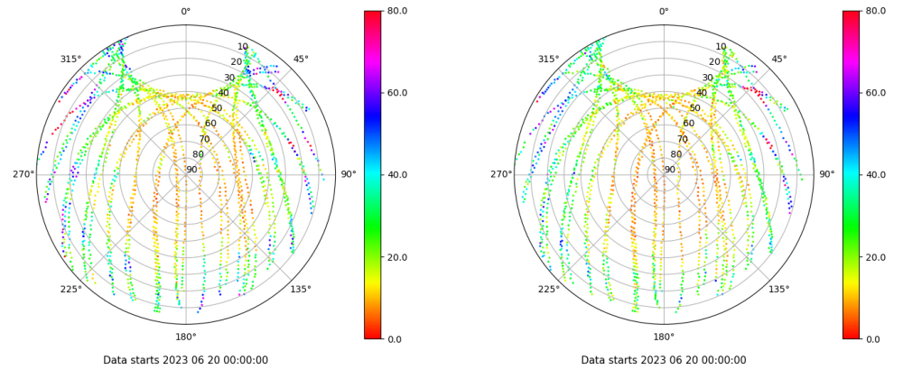
Skyplot for station LPAL. Parameter M1C Data file LPAL00ESP_R_2023171.xtr Skyplot for station LPAL. Parameter M2C Data file LPAL00ESP_R_2023171.xtr
