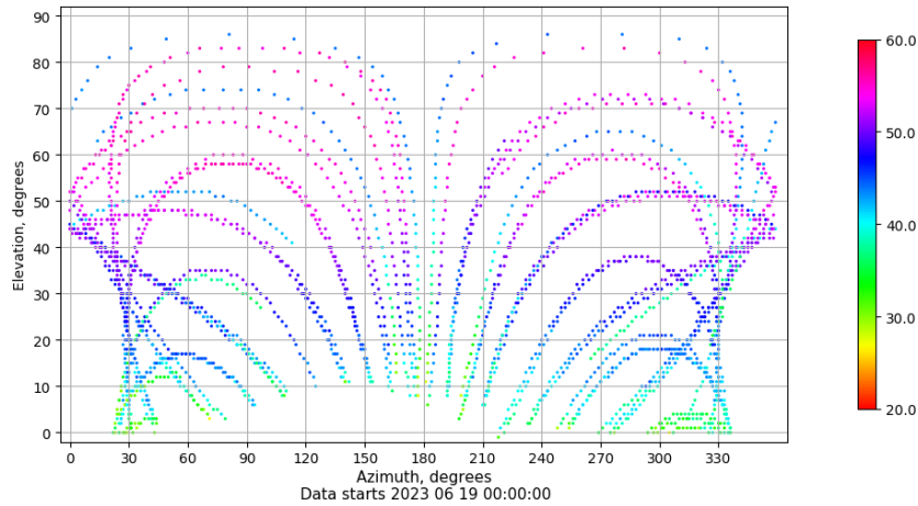
Azimuth-elevation plot for station LPAL. Signal to Noise S1C Data file LPAL00ESP_R_2023170.xtr
