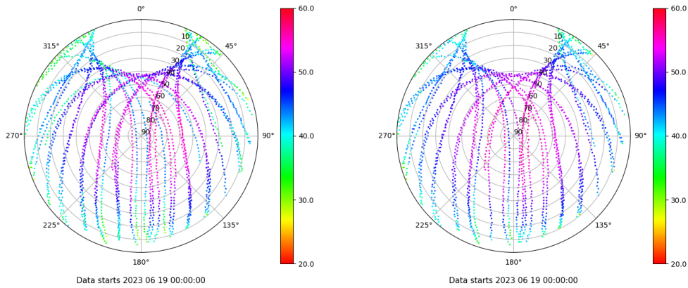
Skyplot for station LPAL. Signal to Noise S1C Data file LPAL00ESP_R_2023170.xtr Skyplot for station LPAL. Signal to Noise S2C Data file LPAL00ESP_R_2023170.xtr
