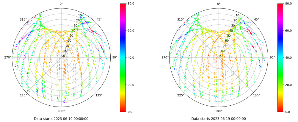
Skyplot for station LPAL. Parameter M1C Data file LPAL00ESP_R_2023170.xtr Skyplot for station LPAL. Parameter M2C Data file LPAL00ESP_R_2023170.xtr
