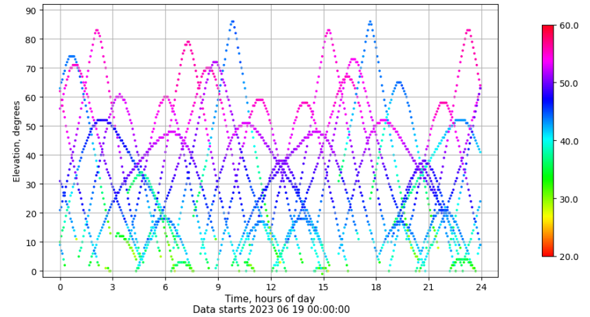
Time-elevation plot for station LPAL. Signal to Noise S1C Data file LPAL00ESP_R_2023170.xtr
