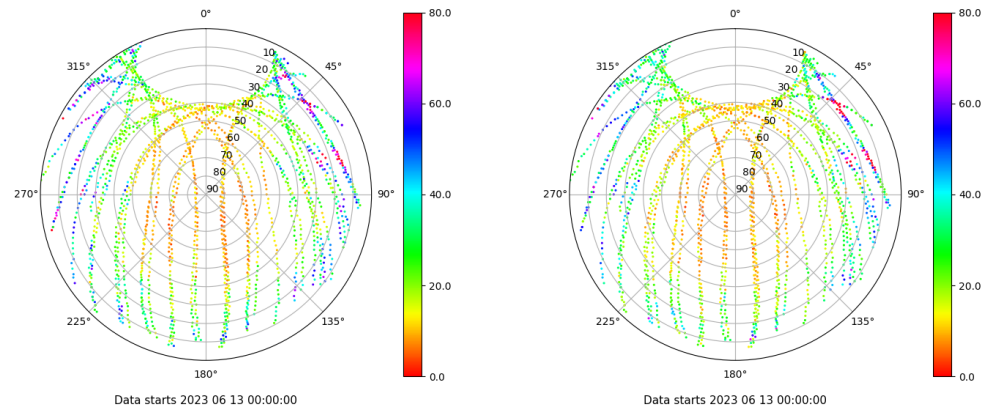
Skyplot for station LPAL. Parameter M1C Data file LPAL00ESP_R_2023164.xtr Skyplot for station LPAL. Parameter M2C Data file LPAL00ESP_R_2023164.xtr
