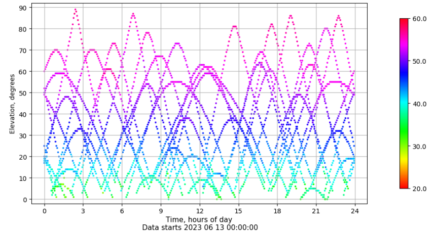
Time-elevation plot for station LPAL. Signal to Noise S1C Data file LPAL00ESP_R_2023164.xtr
