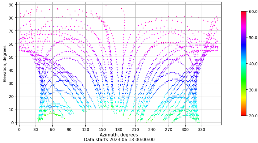
Azimuth-elevation plot for station LPAL. Signal to Noise S1C Data file LPAL00ESP_R_2023164.xtr
