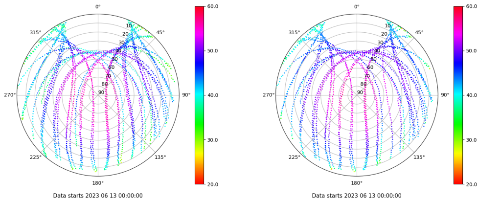
Skyplot for station LPAL. Signal to Noise S1C Data file LPAL00ESP_R_2023164.xtr Skyplot for station LPAL. Signal to Noise S2C Data file LPAL00ESP_R_2023164.xtr
