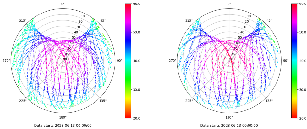
Skyplot for station LPAL. Signal to Noise S1C Data file LPAL00ESP_R_2023164.xtr Skyplot for station LPAL. Signal to Noise S2S Data file LPAL00ESP_R_2023164.xtr
