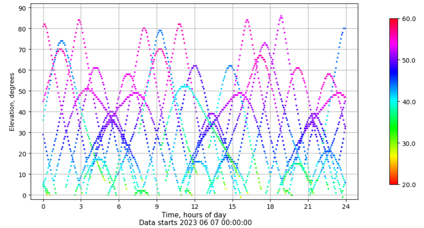
Time-elevation plot for station LPAL. Signal to Noise S1C Data file LPAL00ESP_R_2023158.xtr
