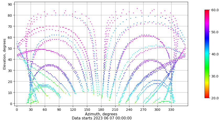
Azimuth-elevation plot for station LPAL. Signal to Noise S1C Data file LPAL00ESP_R_2023158.xtr
