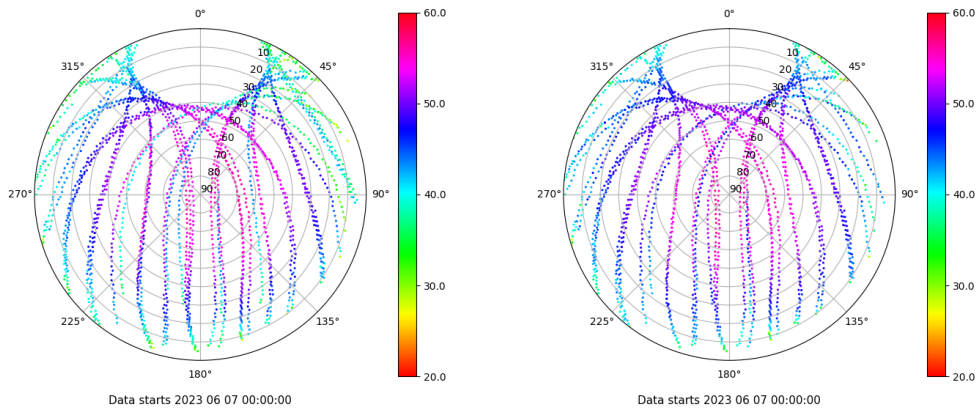
Skyplot for station LPAL. Signal to Noise S1C Data file LPAL00ESP_R_2023158.xtr Skyplot for station LPAL. Signal to Noise S2C Data file LPAL00ESP_R_2023158.xtr
