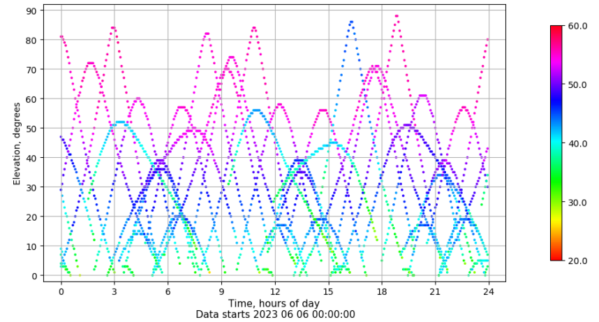
Time-elevation plot for station LPAL. Signal to Noise S1C Data file LPAL00ESP_R_2023157.xtr
