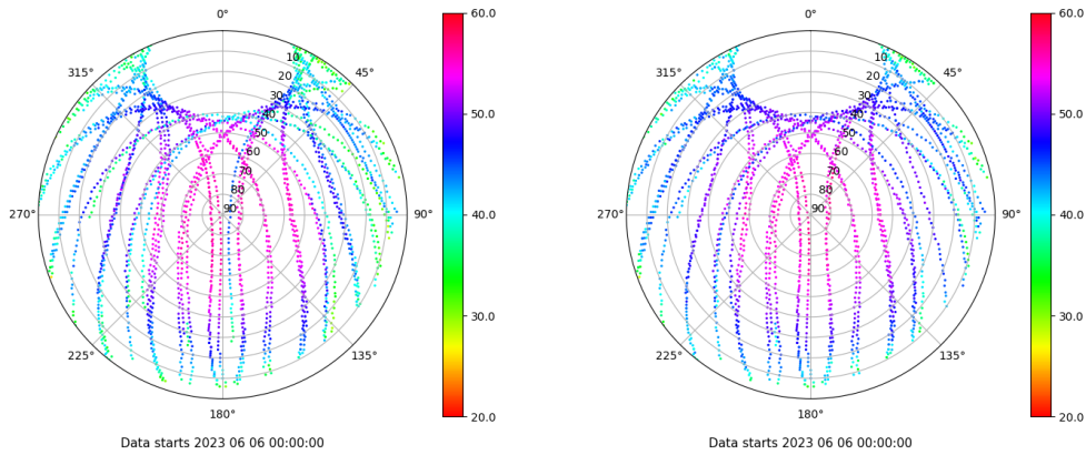
Skyplot for station LPAL. Signal to Noise S1C Data file LPAL00ESP_R_2023157.xtr Skyplot for station LPAL. Signal to Noise S2C Data file LPAL00ESP_R_2023157.xtr
