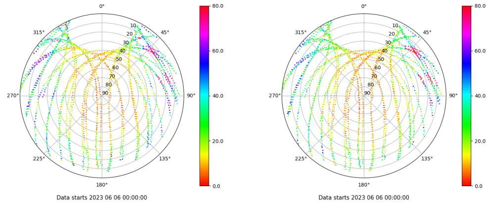
Skyplot for station LPAL. Parameter M1C Data file LPAL00ESP_R_2023157.xtr Skyplot for station LPAL. Parameter M2C Data file LPAL00ESP_R_2023157.xtr
