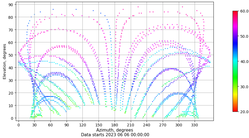
Azimuth-elevation plot for station LPAL. Signal to Noise S1C Data file LPAL00ESP_R_2023157.xtr
