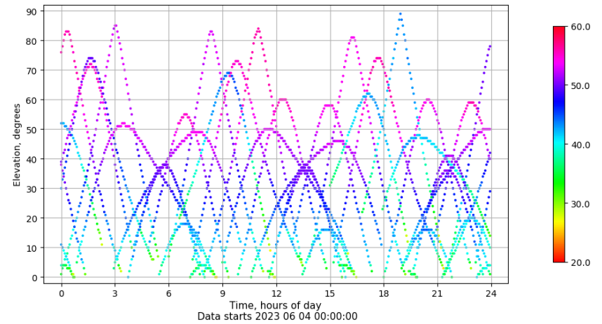
Time-elevation plot for station LPAL. Signal to Noise S1C Data file LPAL00ESP_R_2023155.xtr
