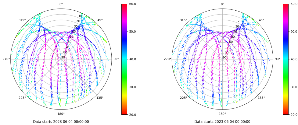
Skyplot for station LPAL. Signal to Noise S1C Data file LPAL00ESP_R_2023155.xtr Skyplot for station LPAL. Signal to Noise S2C Data file LPAL00ESP_R_2023155.xtr
