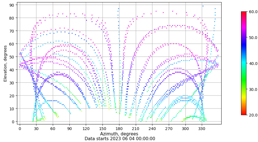
Azimuth-elevation plot for station LPAL. Signal to Noise S1C Data file LPAL00ESP_R_2023155.xtr
