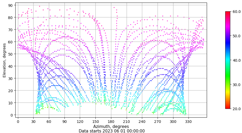
Azimuth-elevation plot for station LPAL. Signal to Noise S1C Data file LPAL00ESP_R_2023152.xtr
