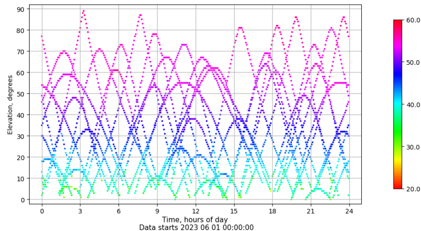
Time-elevation plot for station LPAL. Signal to Noise S1C Data file LPAL00ESP_R_2023152.xtr
