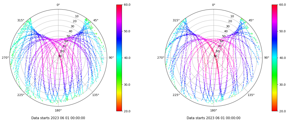
Skyplot for station LPAL. Signal to Noise S1C Data file LPAL00ESP_R_2023152.xtr Skyplot for station LPAL. Signal to Noise S2S Data file LPAL00ESP_R_2023152.xtr
