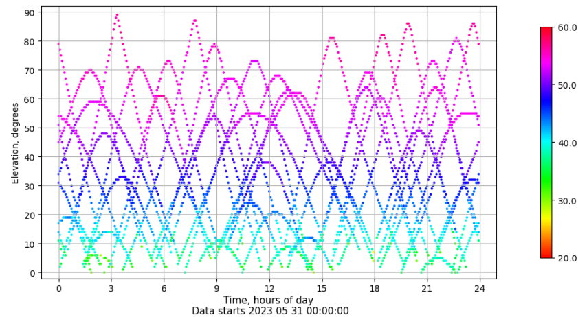
Time-elevation plot for station LPAL. Signal to Noise S1C Data file LPAL00ESP_R_2023151.xtr
