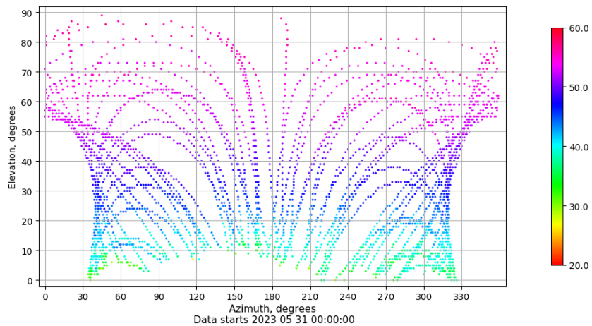
Azimuth-elevation plot for station LPAL. Signal to Noise S1C Data file LPAL00ESP_R_2023151.xtr
