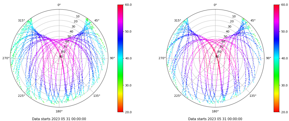
Skyplot for station LPAL. Signal to Noise S1C Data file LPAL00ESP_R_2023151.xtr Skyplot for station LPAL. Signal to Noise S2S Data file LPAL00ESP_R_2023151.xtr
