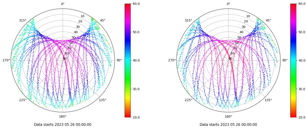
Skyplot for station LPAL. Signal to Noise S1C Data file LPAL00ESP_R_2023146.xtr Skyplot for station LPAL. Signal to Noise S2S Data file LPAL00ESP_R_2023146.xtr
