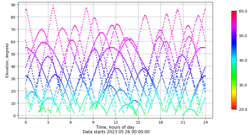
Time-elevation plot for station LPAL. Signal to Noise S1C Data file LPAL00ESP_R_2023146.xtr
