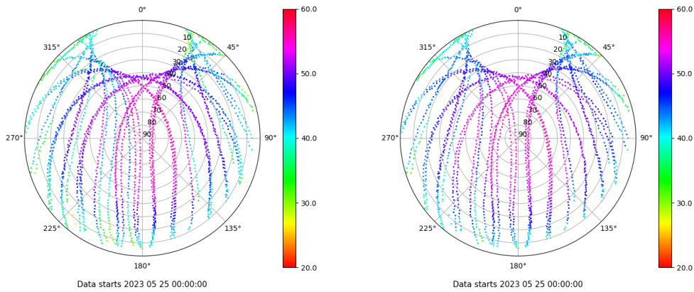
Skyplot for station LPAL. Signal to Noise S1C Data file LPAL00ESP_R_2023145.xtr Skyplot for station LPAL. Signal to Noise S2C Data file LPAL00ESP_R_2023145.xtr
