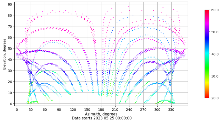
Azimuth-elevation plot for station LPAL. Signal to Noise S1C Data file LPAL00ESP_R_2023145.xtr
