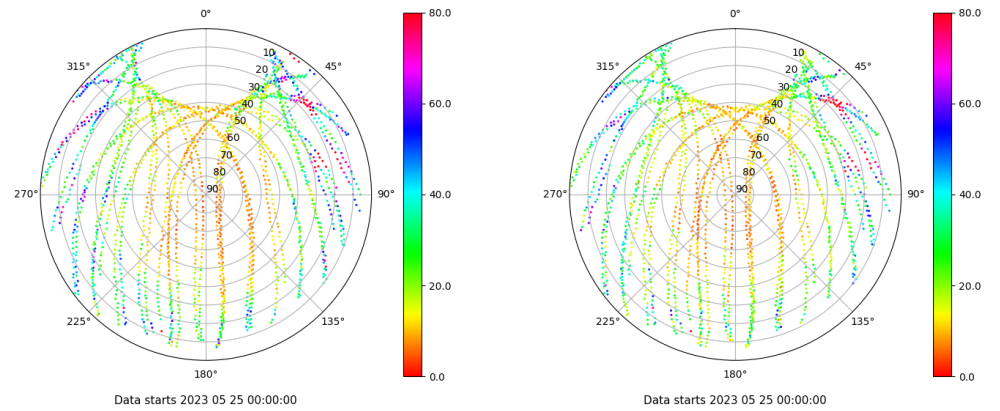
Skyplot for station LPAL. Parameter M1C Data file LPAL00ESP_R_2023145.xtr Skyplot for station LPAL. Parameter M2C Data file LPAL00ESP_R_2023145.xtr
