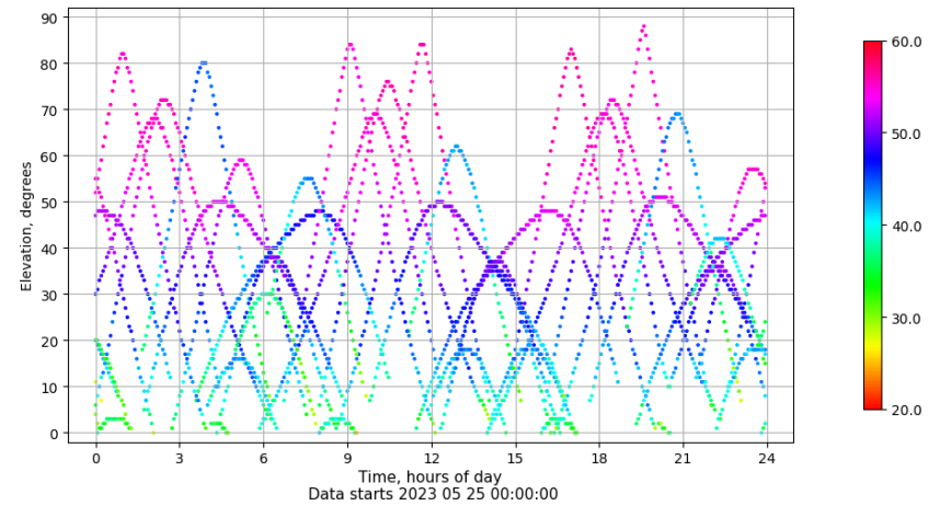
Time-elevation plot for station LPAL. Signal to Noise S1C Data file LPAL00ESP_R_2023145.xtr
