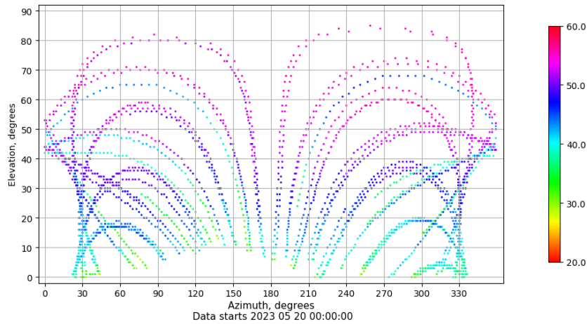
Azimuth-elevation plot for station LPAL. Signal to Noise S1C Data file LPAL00ESP_R_2023140.xtr
