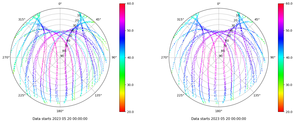
Skyplot for station LPAL. Signal to Noise S1C Data file LPAL00ESP_R_2023140.xtr Skyplot for station LPAL. Signal to Noise S2C Data file LPAL00ESP_R_2023140.xtr
