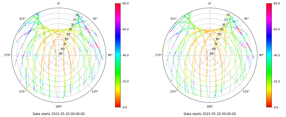
Skyplot for station LPAL. Parameter M1C Data file LPAL00ESP_R_2023140.xtr Skyplot for station LPAL. Parameter M2C Data file LPAL00ESP_R_2023140.xtr
