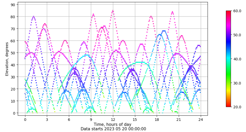
Time-elevation plot for station LPAL. Signal to Noise S1C Data file LPAL00ESP_R_2023140.xtr
