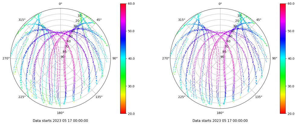
Skyplot for station LPAL. Signal to Noise S1C Data file LPAL00ESP_R_2023137.xtr Skyplot for station LPAL. Signal to Noise S2C Data file LPAL00ESP_R_2023137.xtr
