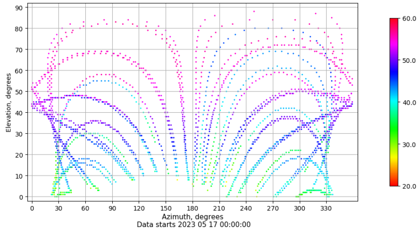
Azimuth-elevation plot for station LPAL. Signal to Noise S1C Data file LPAL00ESP_R_2023137.xtr
