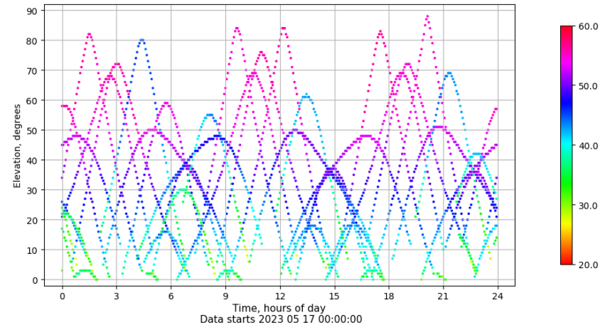
Time-elevation plot for station LPAL. Signal to Noise S1C Data file LPAL00ESP_R_2023137.xtr
