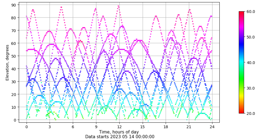
Time-elevation plot for station LPAL. Signal to Noise S1C Data file LPAL00ESP_R_2023134.xtr
