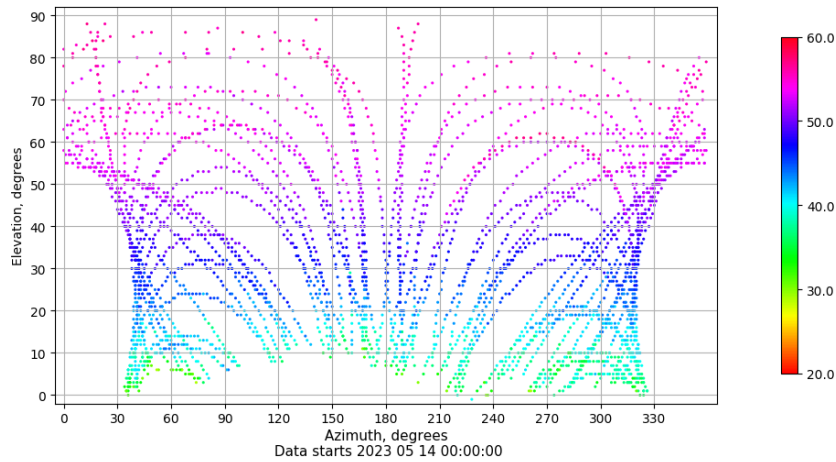
Azimuth-elevation plot for station LPAL. Signal to Noise S1C Data file LPAL00ESP_R_2023134.xtr
