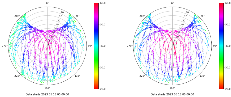
Skyplot for station LPAL. Signal to Noise S1C Data file LPAL00ESP_R_2023133.xtr Skyplot for station LPAL. Signal to Noise S2S Data file LPAL00ESP_R_2023133.xtr
