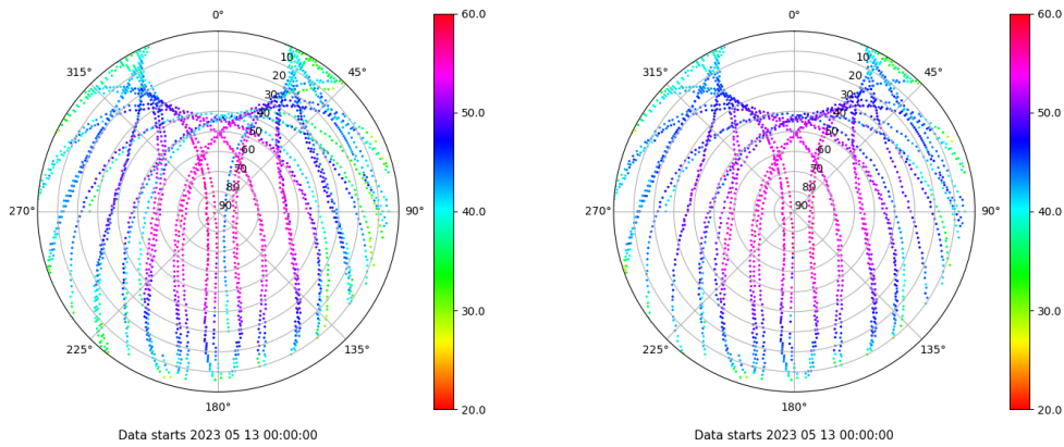
Skyplot for station LPAL. Signal to Noise S1C Data file LPAL00ESP_R_2023133.xtr Skyplot for station LPAL. Signal to Noise S2C Data file LPAL00ESP_R_2023133.xtr
