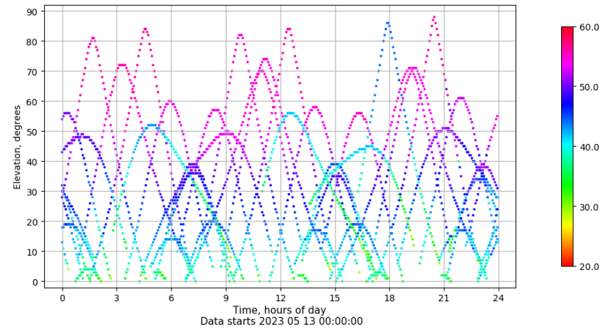
Time-elevation plot for station LPAL. Signal to Noise S1C Data file LPAL00ESP_R_2023133.xtr
