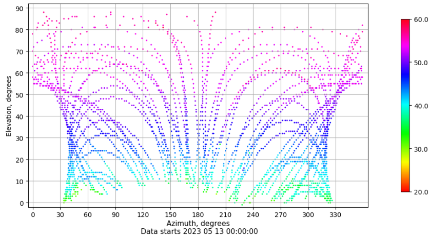
Azimuth-elevation plot for station LPAL. Signal to Noise S1C Data file LPAL00ESP_R_2023133.xtr
