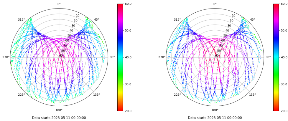
Skyplot for station LPAL. Signal to Noise S1C Data file LPAL00ESP_R_2023131.xtr Skyplot for station LPAL. Signal to Noise S2S Data file LPAL00ESP_R_2023131.xtr
