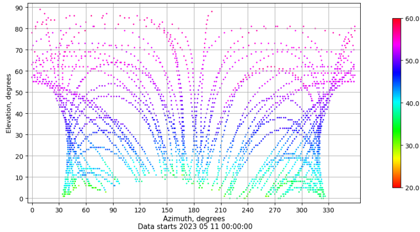
Azimuth-elevation plot for station LPAL. Signal to Noise S1C Data file LPAL00ESP_R_2023131.xtr
