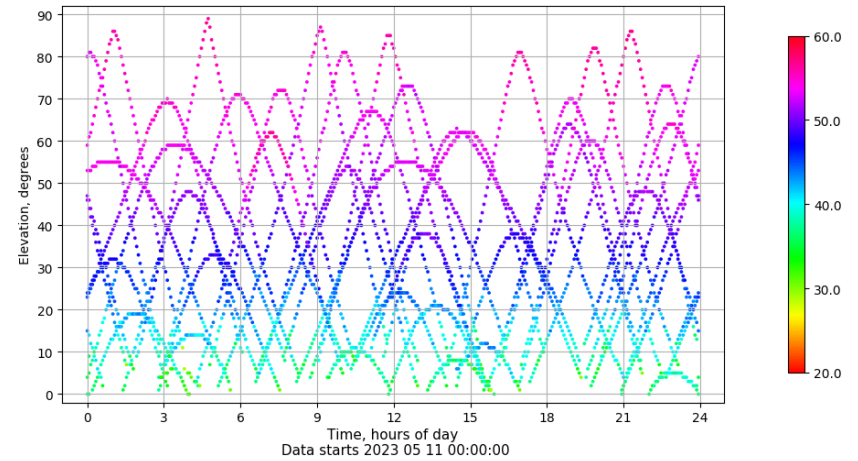
Time-elevation plot for station LPAL. Signal to Noise S1C Data file LPAL00ESP_R_2023131.xtr
