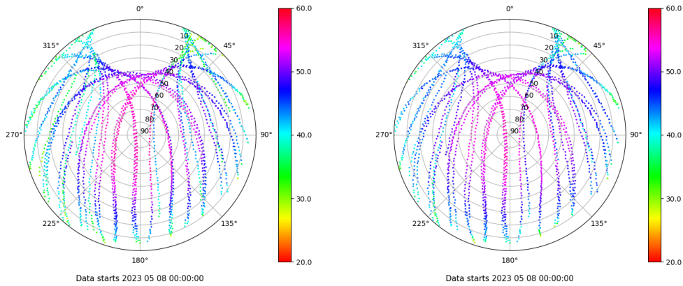
Skyplot for station LPAL. Signal to Noise S1C Data file LPAL00ESP_R_2023128.xtr Skyplot for station LPAL. Signal to Noise S2C Data file LPAL00ESP_R_2023128.xtr
