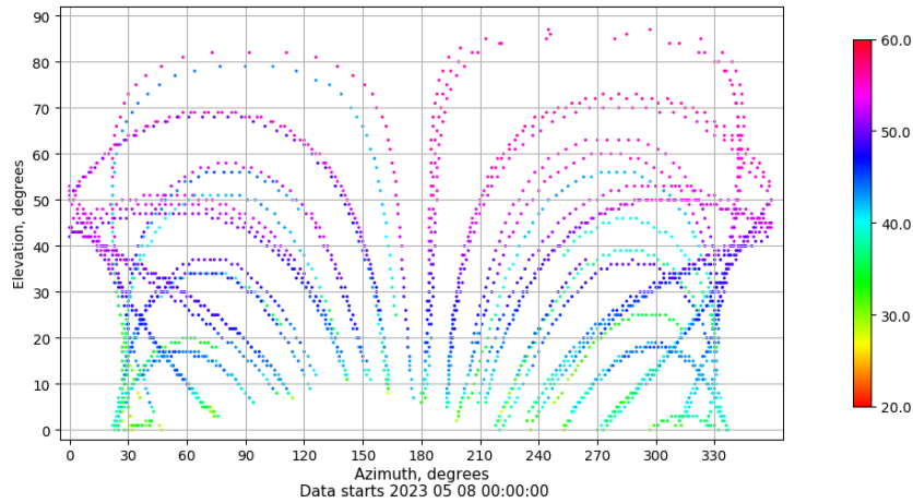
Azimuth-elevation plot for station LPAL. Signal to Noise S1C Data file LPAL00ESP_R_2023128.xtr
