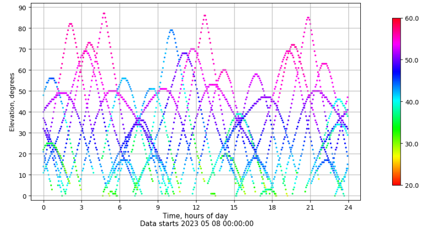
Time-elevation plot for station LPAL. Signal to Noise S1C Data file LPAL00ESP_R_2023128.xtr
