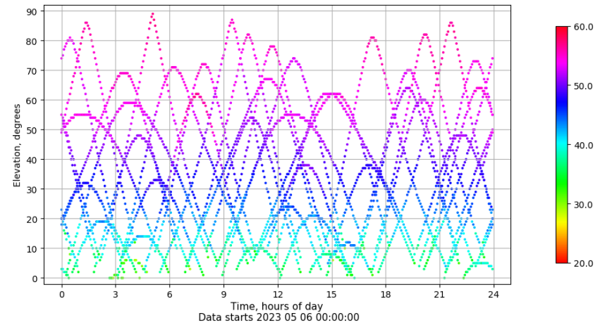
Time-elevation plot for station LPAL. Signal to Noise S1C Data file LPAL00ESP_R_2023126.xtr
