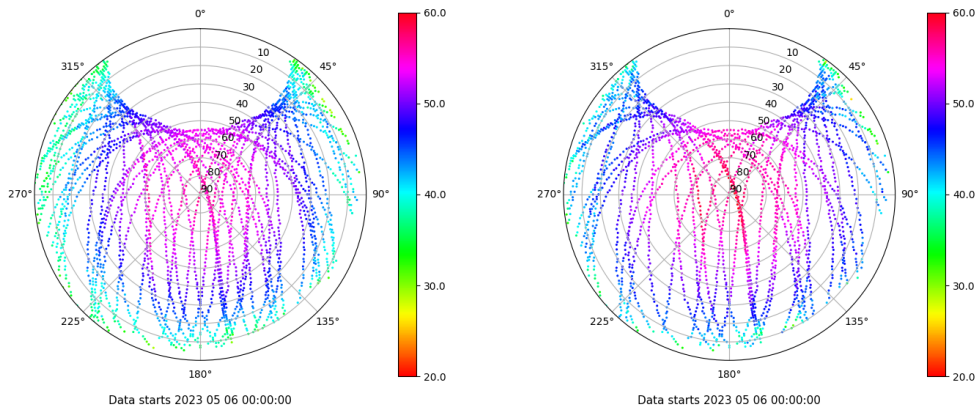
Skyplot for station LPAL. Signal to Noise S1C Data file LPAL00ESP_R_2023126.xtr Skyplot for station LPAL. Signal to Noise S2S Data file LPAL00ESP_R_2023126.xtr
