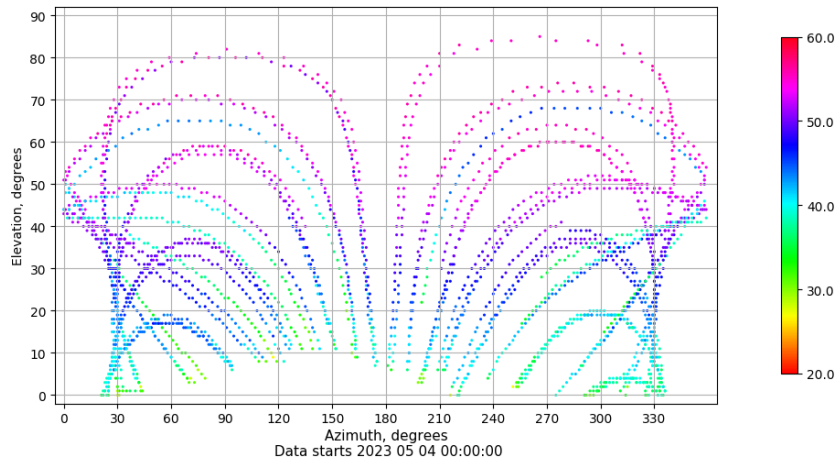
Azimuth-elevation plot for station LPAL. Signal to Noise S1C Data file LPAL00ESP_R_2023124.xtr
