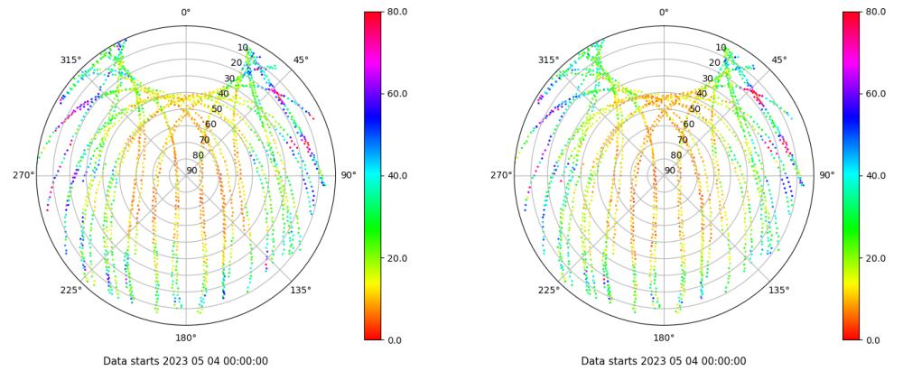
Skyplot for station LPAL. Parameter M1C Data file LPAL00ESP_R_2023124.xtr Skyplot for station LPAL. Parameter M2C Data file LPAL00ESP_R_2023124.xtr
