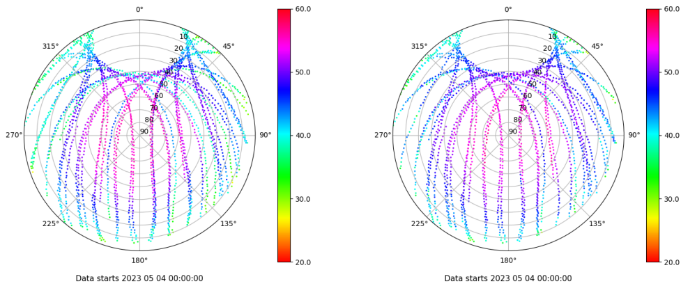
Skyplot for station LPAL. Signal to Noise S1C Data file LPAL00ESP_R_2023124.xtr Skyplot for station LPAL. Signal to Noise S2C Data file LPAL00ESP_R_2023124.xtr
