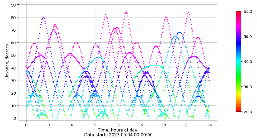
Time-elevation plot for station LPAL. Signal to Noise S1C Data file LPAL00ESP_R_2023124.xtr
