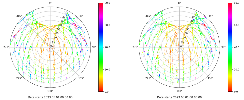
Skyplot for station LPAL. Parameter M1C Data file LPAL00ESP_R_2023121.xtr Skyplot for station LPAL. Parameter M2C Data file LPAL00ESP_R_2023121.xtr
