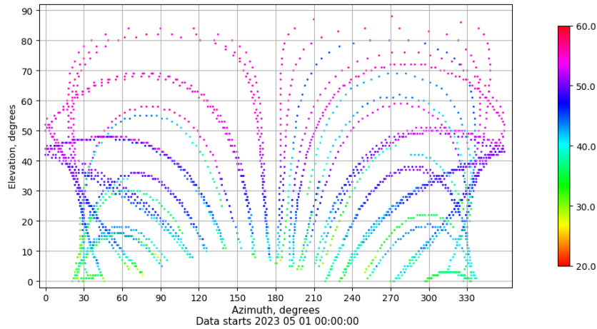
Azimuth-elevation plot for station LPAL. Signal to Noise S1C Data file LPAL00ESP_R_2023121.xtr
