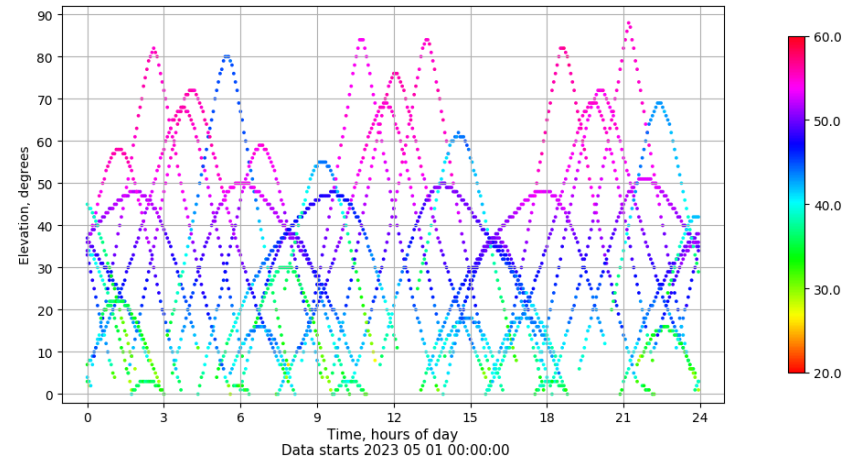
Time-elevation plot for station LPAL. Signal to Noise S1C Data file LPAL00ESP_R_2023121.xtr
