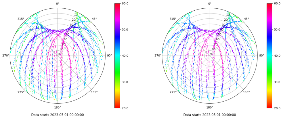
Skyplot for station LPAL. Signal to Noise S1C Data file LPAL00ESP_R_2023121.xtr Skyplot for station LPAL. Signal to Noise S2C Data file LPAL00ESP_R_2023121.xtr
