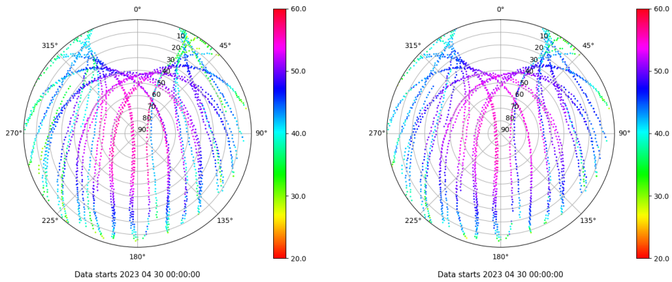
Skyplot for station LPAL. Signal to Noise S1C Data file LPAL00ESP_R_2023120.xtr Skyplot for station LPAL. Signal to Noise S2C Data file LPAL00ESP_R_2023120.xtr
