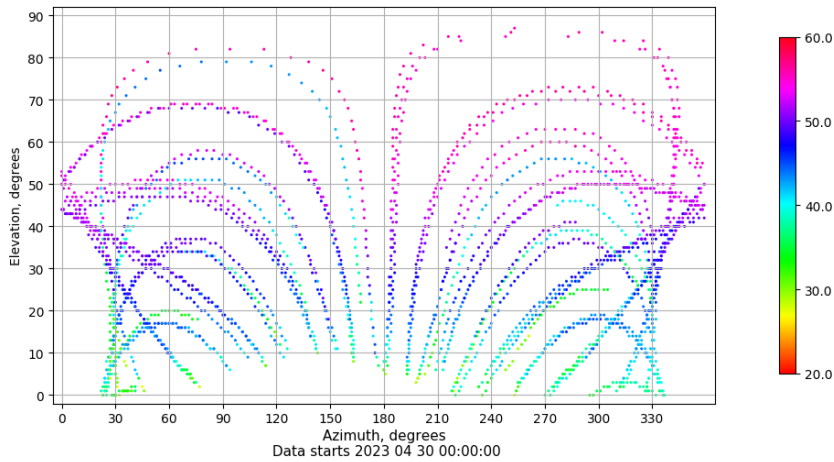
Azimuth-elevation plot for station LPAL. Signal to Noise S1C Data file LPAL00ESP_R_2023120.xtr
