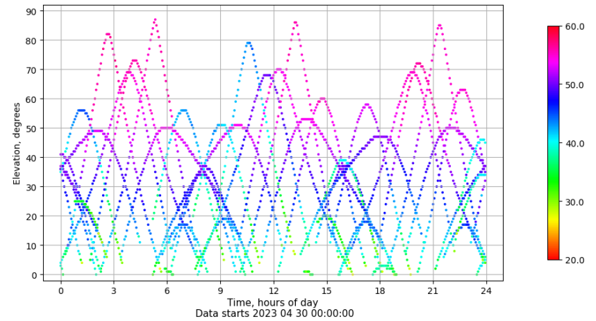
Time-elevation plot for station LPAL. Signal to Noise S1C Data file LPAL00ESP_R_2023120.xtr
