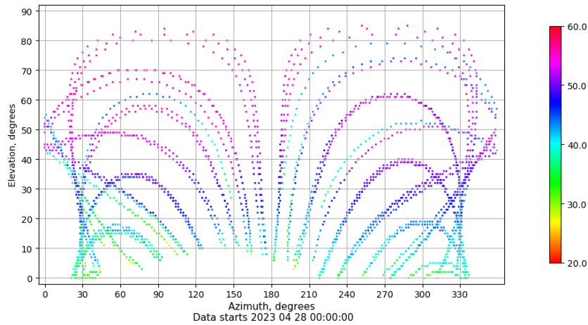
Azimuth-elevation plot for station LPAL. Signal to Noise S1C Data file LPAL00ESP_R_2023118.xtr
