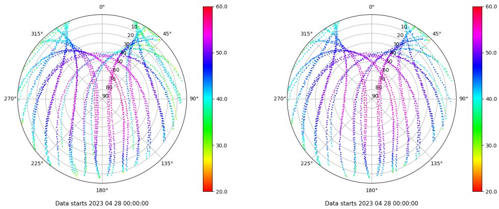
Skyplot for station LPAL. Signal to Noise S1C Data file LPAL00ESP_R_2023118.xtr Skyplot for station LPAL. Signal to Noise S2C Data file LPAL00ESP_R_2023118.xtr
