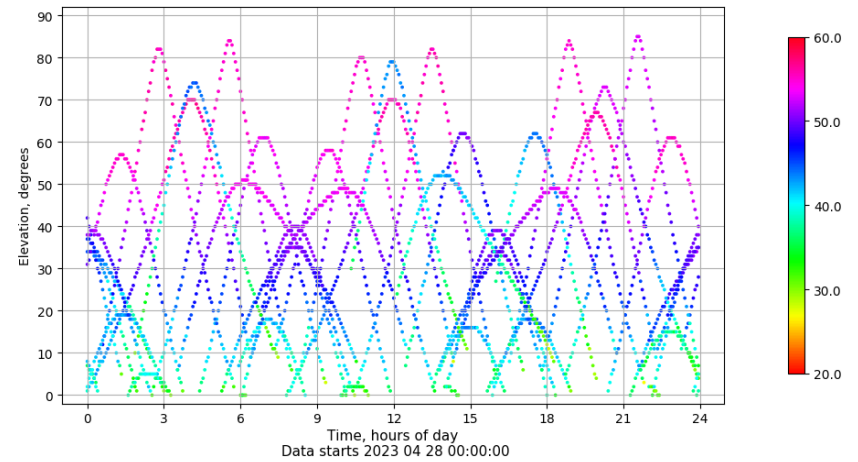
Time-elevation plot for station LPAL. Signal to Noise S1C Data file LPAL00ESP_R_2023118.xtr
