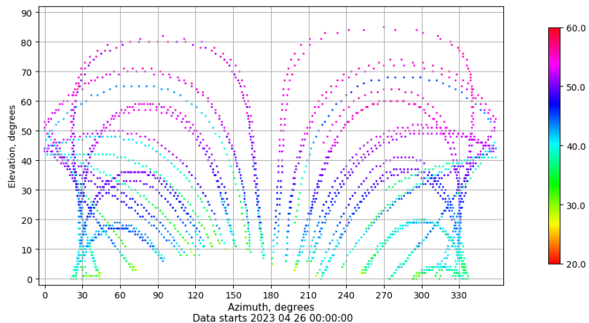
Azimuth-elevation plot for station LPAL. Signal to Noise S1C Data file LPAL00ESP_R_2023116.xtr
