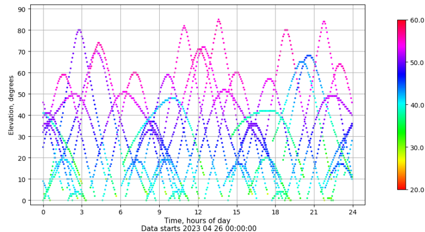
Time-elevation plot for station LPAL. Signal to Noise S1C Data file LPAL00ESP_R_2023116.xtr
