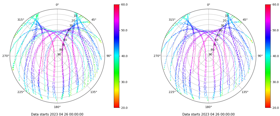
Skyplot for station LPAL. Signal to Noise S1C Data file LPAL00ESP_R_2023116.xtr Skyplot for station LPAL. Signal to Noise S2C Data file LPAL00ESP_R_2023116.xtr
