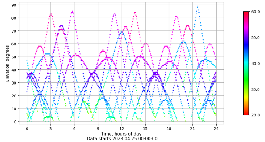
Time-elevation plot for station LPAL. Signal to Noise S1C Data file LPAL00ESP_R_2023115.xtr
