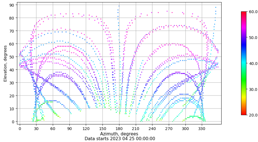
Azimuth-elevation plot for station LPAL. Signal to Noise S1C Data file LPAL00ESP_R_2023115.xtr
