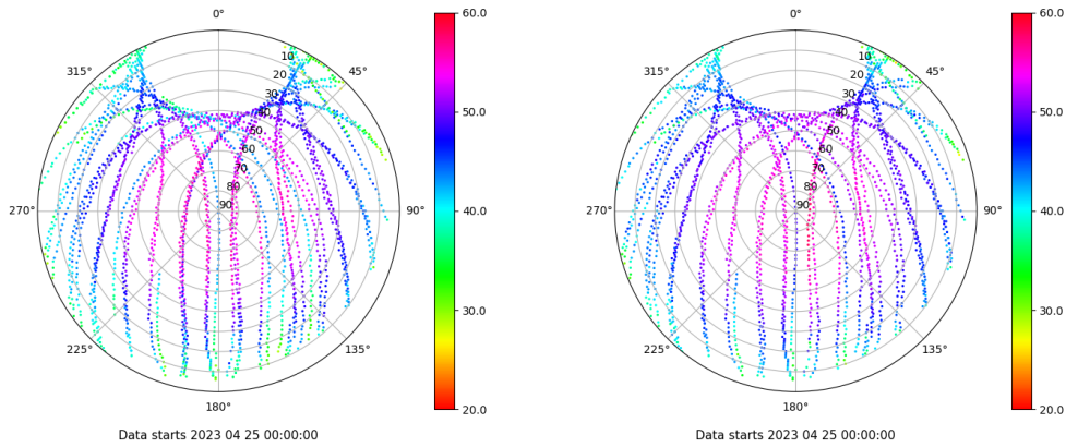
Skyplot for station LPAL. Signal to Noise S1C Data file LPAL00ESP_R_2023115.xtr Skyplot for station LPAL. Signal to Noise S2C Data file LPAL00ESP_R_2023115.xtr
