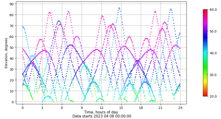
Time-elevation plot for station LPAL. Signal to Noise S1C Data file LPAL00ESP_R_2023098.xtr
