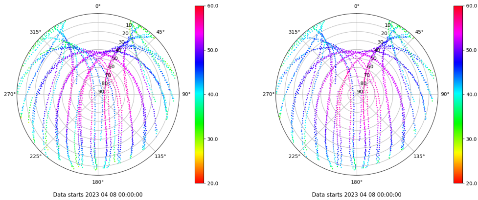
Skyplot for station LPAL. Signal to Noise S1C Data file LPAL00ESP_R_2023098.xtr Skyplot for station LPAL. Signal to Noise S2C Data file LPAL00ESP_R_2023098.xtr
