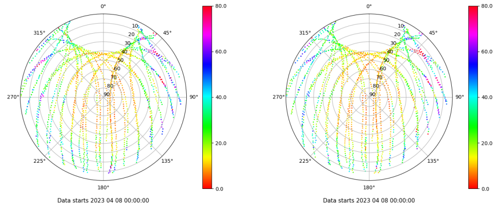
Skyplot for station LPAL. Parameter M1C Data file LPAL00ESP_R_2023098.xtr Skyplot for station LPAL. Parameter M2C Data file LPAL00ESP_R_2023098.xtr
