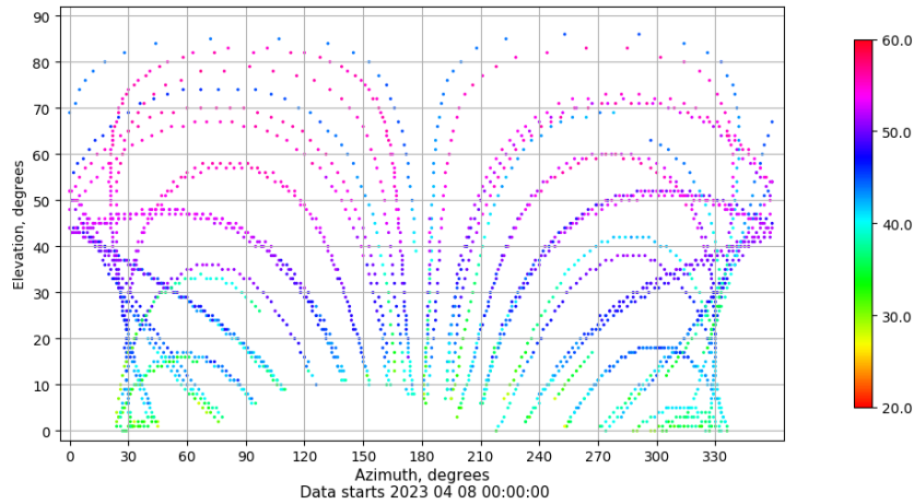
Azimuth-elevation plot for station LPAL. Signal to Noise S1C Data file LPAL00ESP_R_2023098.xtr
