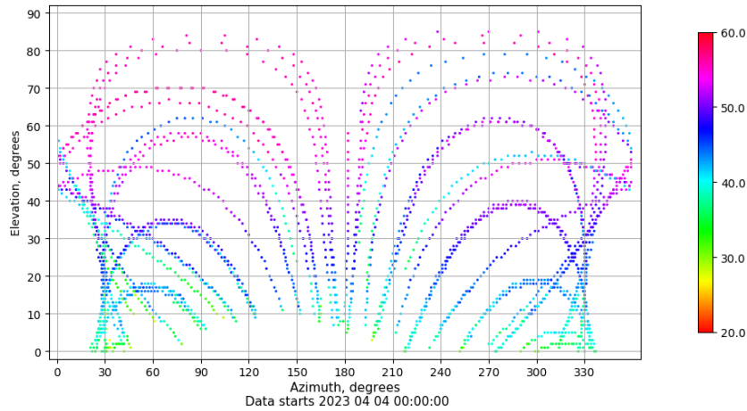
Azimuth-elevation plot for station LPAL. Signal to Noise S1C Data file LPAL00ESP_R_2023094.xtr
