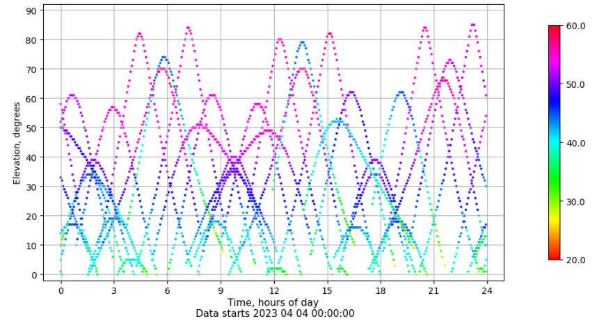
Time-elevation plot for station LPAL. Signal to Noise S1C Data file LPAL00ESP_R_2023094.xtr
