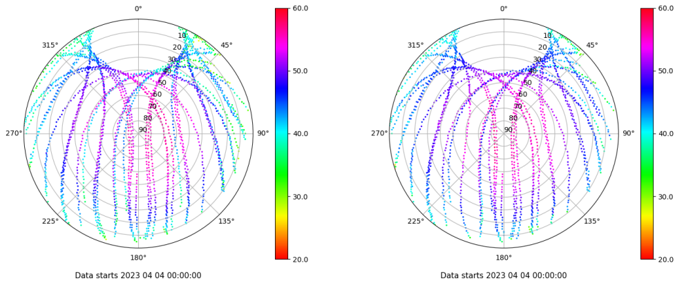
Skyplot for station LPAL. Signal to Noise S1C Data file LPAL00ESP_R_2023094.xtr Skyplot for station LPAL. Signal to Noise S2C Data file LPAL00ESP_R_2023094.xtr
