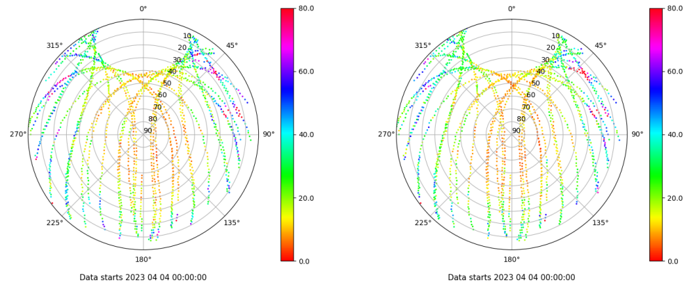
Skyplot for station LPAL. Parameter M1C Data file LPAL00ESP_R_2023094.xtr Skyplot for station LPAL. Parameter M2C Data file LPAL00ESP_R_2023094.xtr
