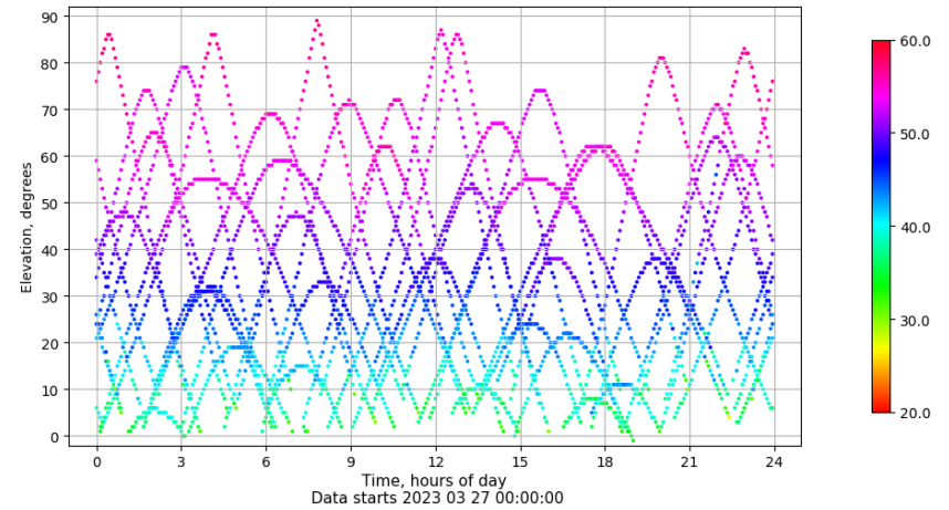
Time-elevation plot for station LPAL. Signal to Noise S1C Data file LPAL00ESP_R_2023086.xtr
