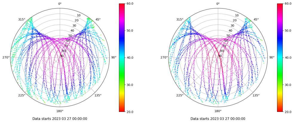
Skyplot for station LPAL. Signal to Noise S1C Data file LPAL00ESP_R_2023086.xtr Skyplot for station LPAL. Signal to Noise S2S Data file LPAL00ESP_R_2023086.xtr
