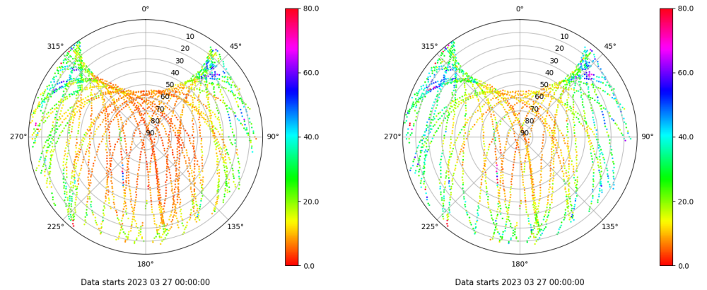
Skyplot for station LPAL. Parameter M1C Data file LPAL00ESP_R_2023086.xtr Skyplot for station LPAL. Parameter M2S Data file LPAL00ESP_R_2023086.xtr
