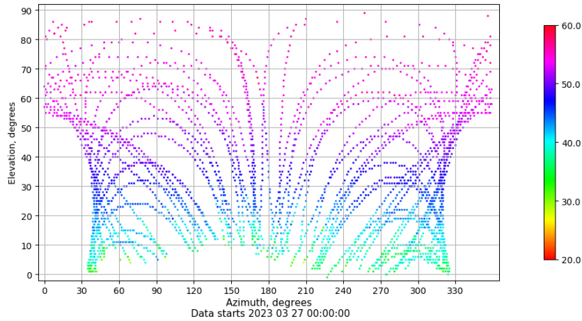
Azimuth-elevation plot for station LPAL. Signal to Noise S1C Data file LPAL00ESP_R_2023086.xtr
