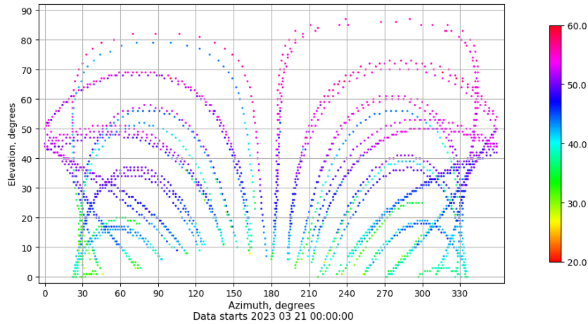
Azimuth-elevation plot for station LPAL. Signal to Noise S1C Data file LPAL00ESP_R_2023080.xtr
