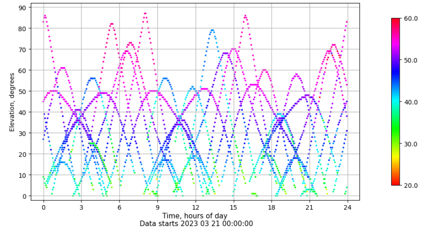
Time-elevation plot for station LPAL. Signal to Noise S1C Data file LPAL00ESP_R_2023080.xtr
