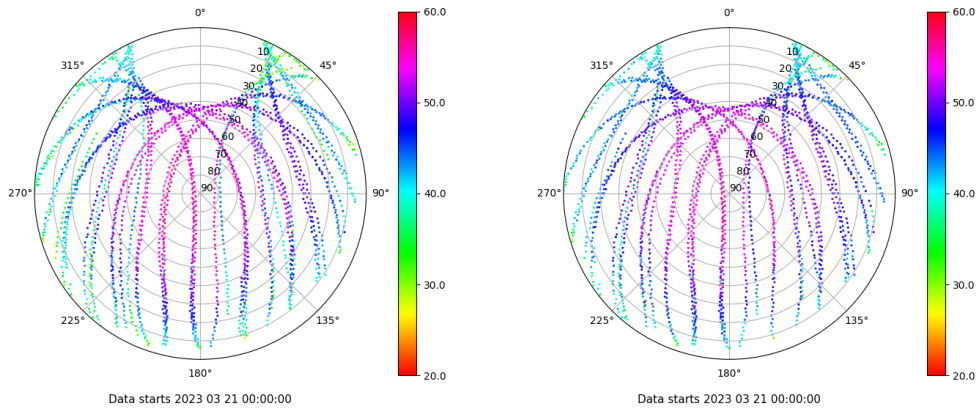
Skyplot for station LPAL. Signal to Noise S1C Data file LPAL00ESP_R_2023080.xtr Skyplot for station LPAL. Signal to Noise S2C Data file LPAL00ESP_R_2023080.xtr
