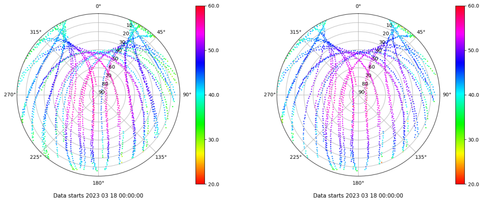
Skyplot for station LPAL. Signal to Noise S1C Data file LPAL00ESP_R_2023077.xtr Skyplot for station LPAL. Signal to Noise S2C Data file LPAL00ESP_R_2023077.xtr
