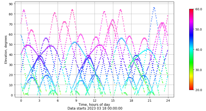
Time-elevation plot for station LPAL. Signal to Noise S1C Data file LPAL00ESP_R_2023077.xtr
