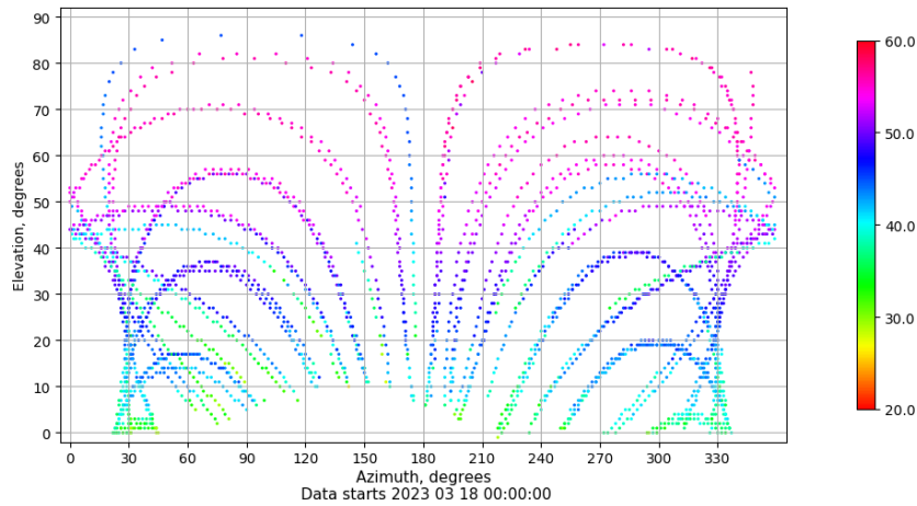
Azimuth-elevation plot for station LPAL. Signal to Noise S1C Data file LPAL00ESP_R_2023077.xtr
