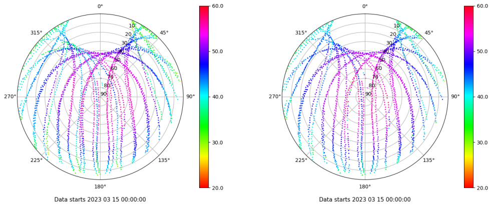
Skyplot for station LPAL. Signal to Noise S1C Data file LPAL00ESP_R_2023074.xtr Skyplot for station LPAL. Signal to Noise S2C Data file LPAL00ESP_R_2023074.xtr
