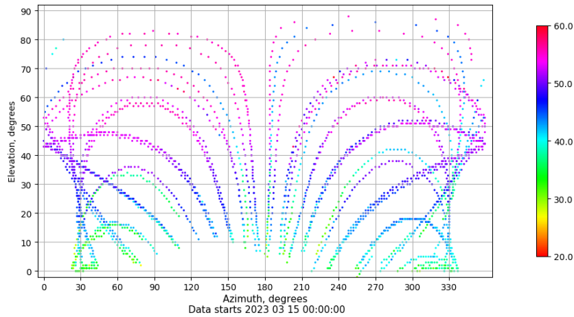
Azimuth-elevation plot for station LPAL. Signal to Noise S1C Data file LPAL00ESP_R_2023074.xtr
