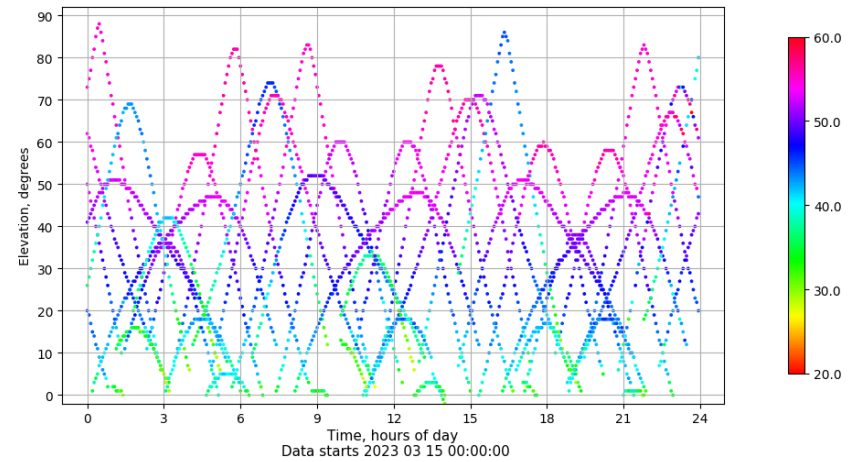
Time-elevation plot for station LPAL. Signal to Noise S1C Data file LPAL00ESP_R_2023074.xtr
