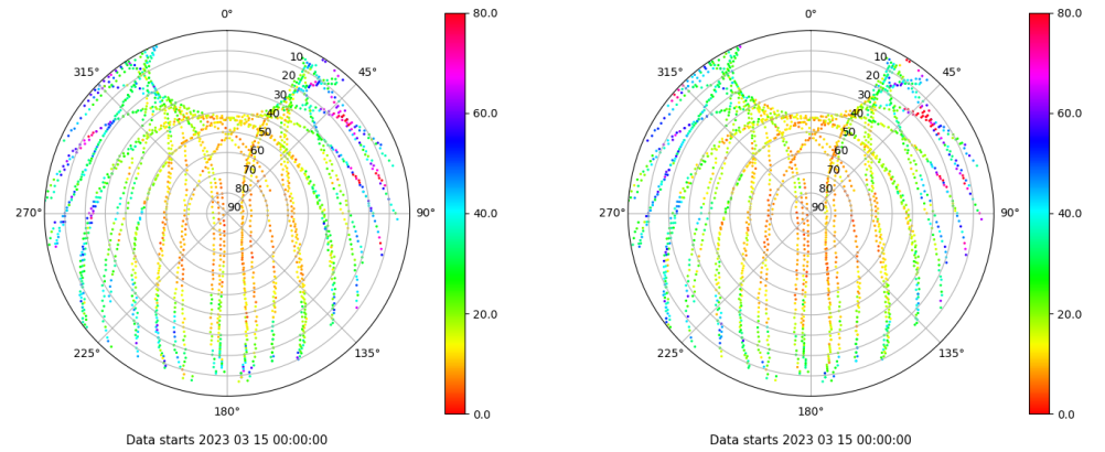
Skyplot for station LPAL. Parameter M1C Data file LPAL00ESP_R_2023074.xtr Skyplot for station LPAL. Parameter M2C Data file LPAL00ESP_R_2023074.xtr
