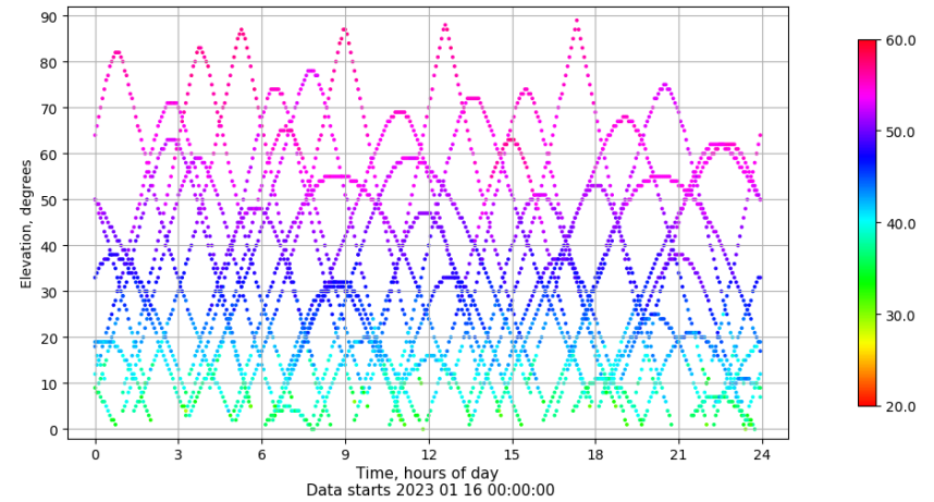
Time-elevation plot for station LPAL. Signal to Noise S1C Data file LPAL00ESP_R_2023016.xtr
