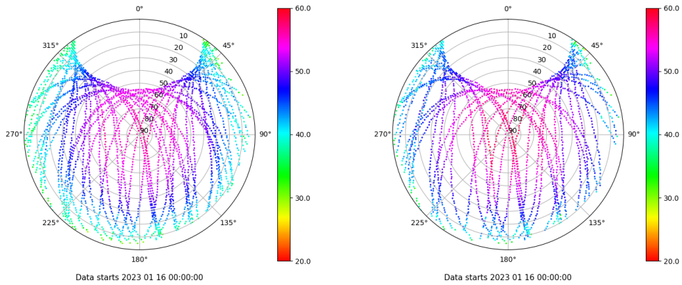
Skyplot for station LPAL. Signal to Noise S1C Data file LPAL00ESP_R_2023016.xtr Skyplot for station LPAL. Signal to Noise S2S Data file LPAL00ESP_R_2023016.xtr
