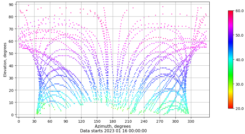
Azimuth-elevation plot for station LPAL. Signal to Noise S1C Data file LPAL00ESP_R_2023016.xtr
