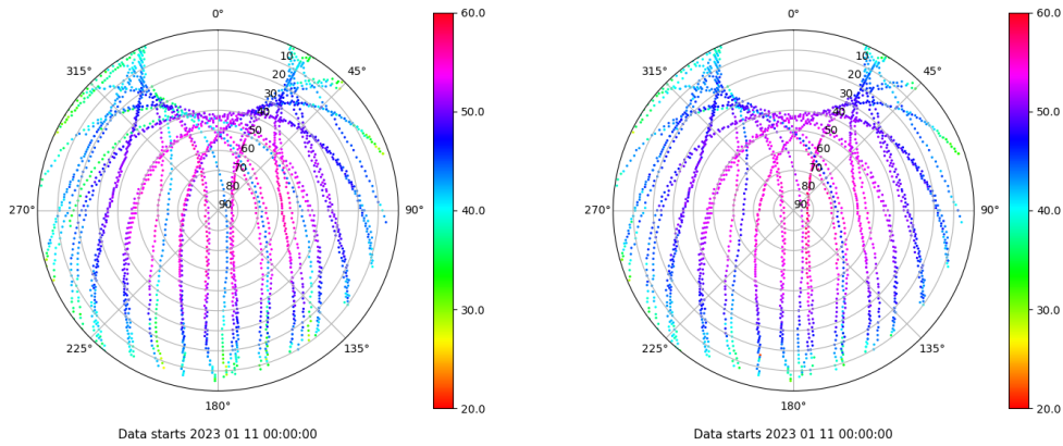
Skyplot for station LPAL. Signal to Noise S1C Data file LPAL00ESP_R_20230111.xtr Skyplot for station LPAL. Signal to Noise S2C Data file LPAL00ESP_R_20230111.xtr
