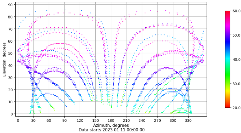
Azimuth-elevation plot for station LPAL. Signal to Noise S1C Data file LPAL00ESP_R_20230111.xtr
