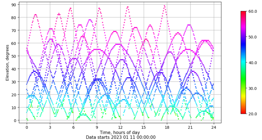
Time-elevation plot for station LPAL. Signal to Noise S1C Data file LPAL00ESP_R_2023011.xtr
