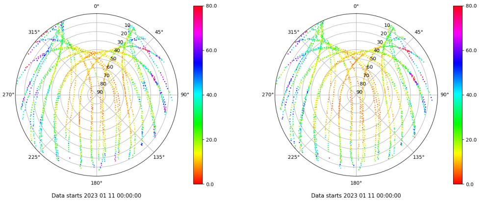
Skyplot for station LPAL. Parameter M1C Data file LPAL00ESP_R_20230111.xtr Skyplot for station LPAL. Parameter M2C Data file LPAL00ESP_R_20230111.xtr
