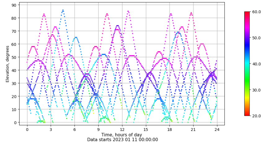
Time-elevation plot for station LPAL. Signal to Noise S1C Data file LPAL00ESP_R_20230111.xtr
