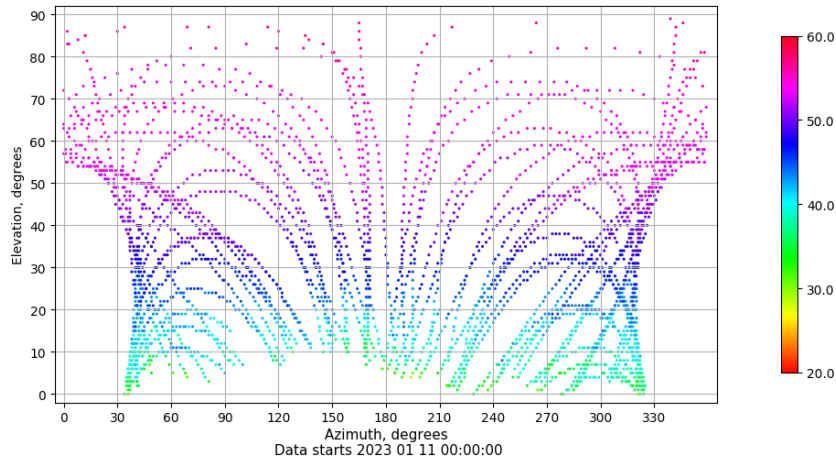
Azimuth-elevation plot for station LPAL. Signal to Noise S1C Data file LPAL00ESP_R_2023011.xtr
