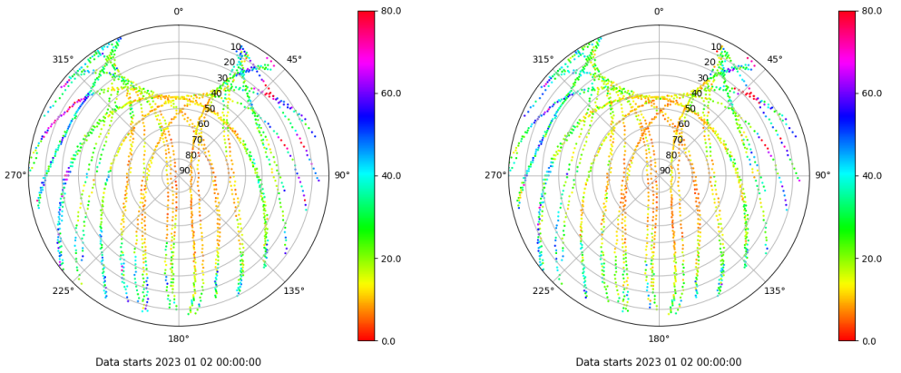
Skyplot for station LPAL. Parameter M1C Data file LPAL00ESP_R_2023002.xtr Skyplot for station LPAL. Parameter M2C Data file LPAL00ESP_R_2023002.xtr
