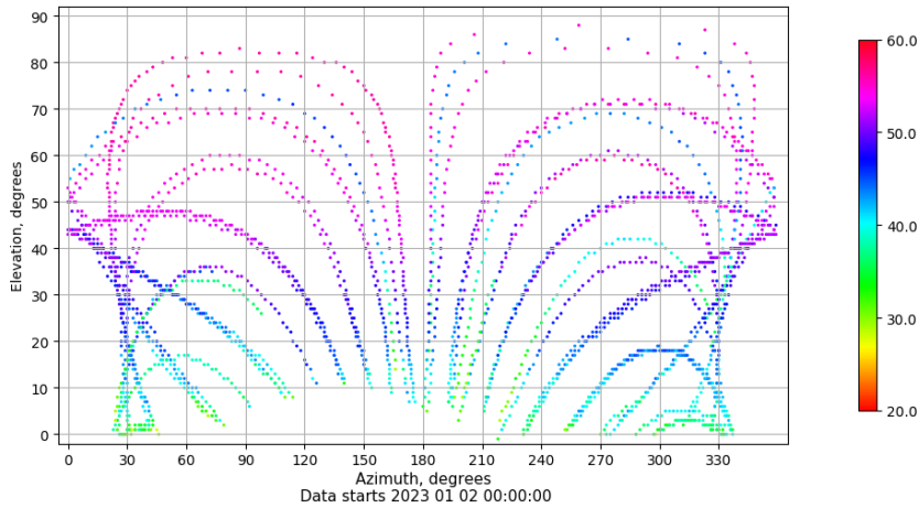
Azimuth-elevation plot for station LPAL. Signal to Noise S1C Data file LPAL00ESP_R_2023002.xtr
