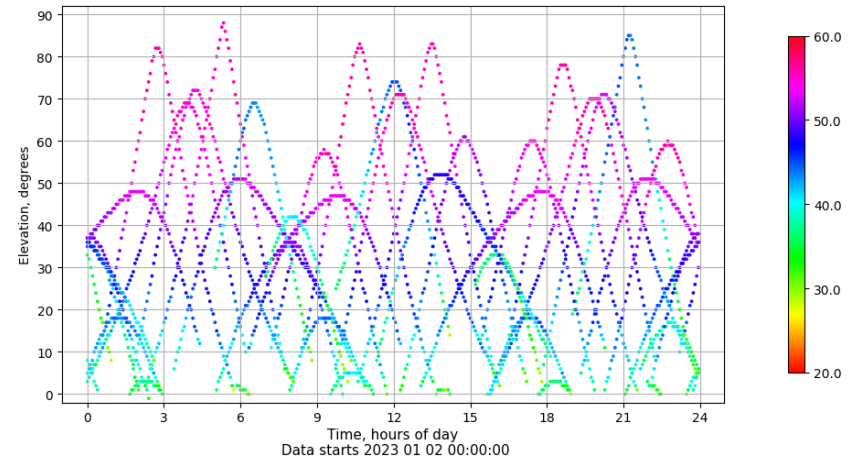
Time-elevation plot for station LPAL. Signal to Noise S1C Data file LPAL00ESP_R_2023002.xtr
