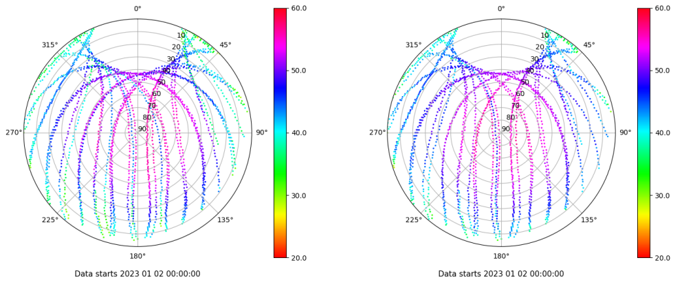
Skyplot for station LPAL. Signal to Noise S1C Data file LPAL00ESP_R_2023002.xtr Skyplot for station LPAL. Signal to Noise S2C Data file LPAL00ESP_R_2023002.xtr
