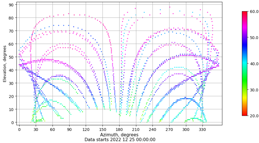
Azimuth-elevation plot for station LPAL. Signal to Noise S1C Data file LPAL00ESP_R_2022359.xtr
