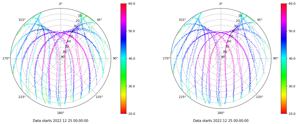
Skyplot for station LPAL. Signal to Noise S1C Data file LPAL00ESP_R_2022359.xtr Skyplot for station LPAL. Signal to Noise S2C Data file LPAL00ESP_R_2022359.xtr
