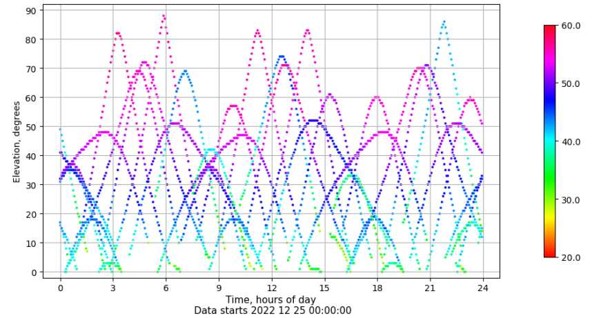
Time-elevation plot for station LPAL. Signal to Noise S1C Data file LPAL00ESP_R_2022359.xtr
