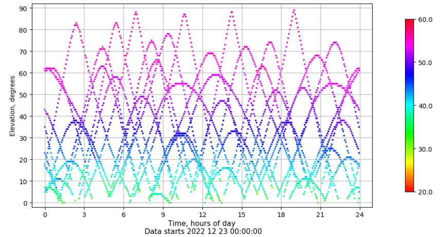
Time-elevation plot for station LPAL. Signal to Noise S1C Data file LPAL00ESP_R_2022357.xtr
