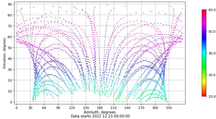
Azimuth-elevation plot for station LPAL. Signal to Noise S1C Data file LPAL00ESP_R_2022357.xtr
