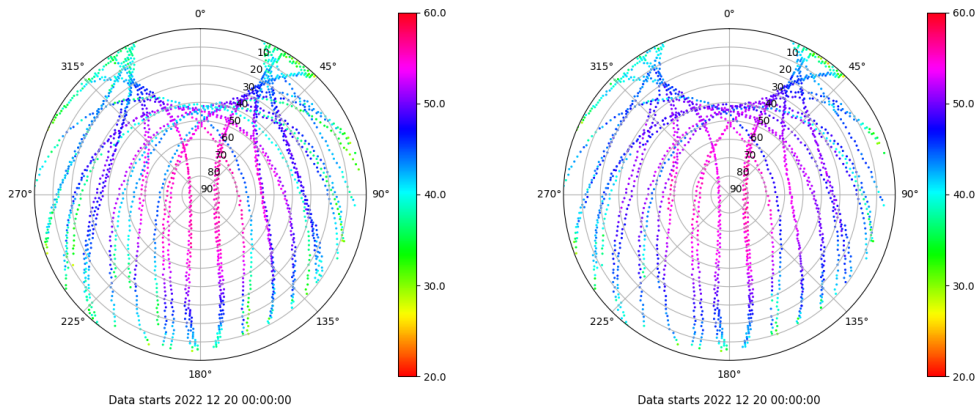
Skyplot for station LPAL. Signal to Noise S1C Data file LPAL00ESP_R_2022354.xtr Skyplot for station LPAL. Signal to Noise S2C Data file LPAL00ESP_R_2022354.xtr
