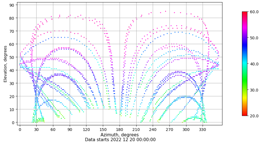
Azimuth-elevation plot for station LPAL. Signal to Noise S1C Data file LPAL00ESP_R_2022354.xtr
