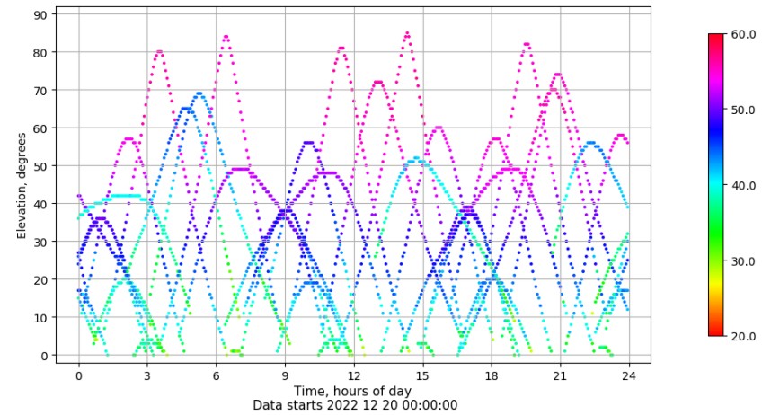
Time-elevation plot for station LPAL. Signal to Noise S1C Data file LPAL00ESP_R_2022354.xtr
