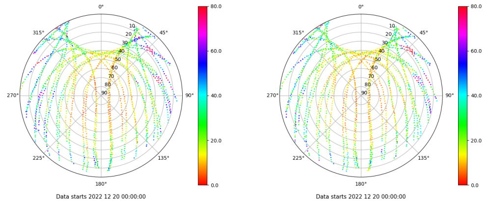
Skyplot for station LPAL. Parameter M1C Data file LPAL00ESP_R_2022354.xtr Skyplot for station LPAL. Parameter M2C Data file LPAL00ESP_R_2022354.xtr
