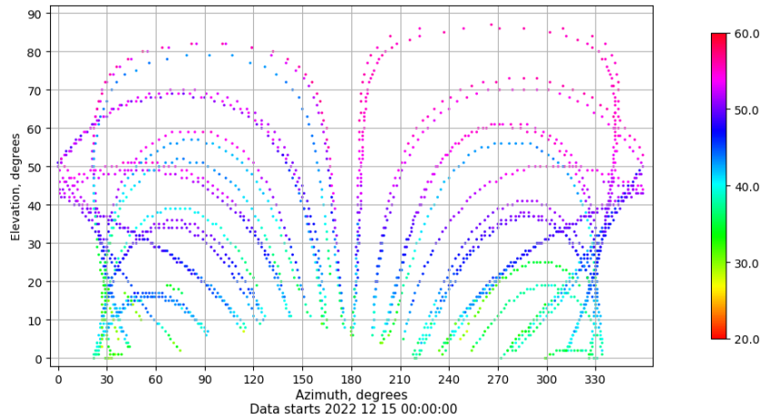
Azimuth-elevation plot for station LPAL. Signal to Noise S1C Data file LPAL00ESP_R_2022349.xtr
