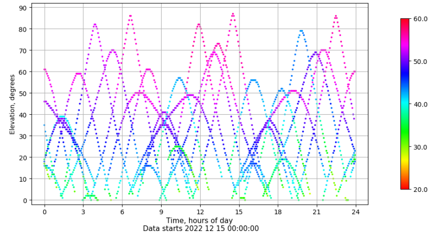
Time-elevation plot for station LPAL. Signal to Noise S1C Data file LPAL00ESP_R_2022349.xtr
